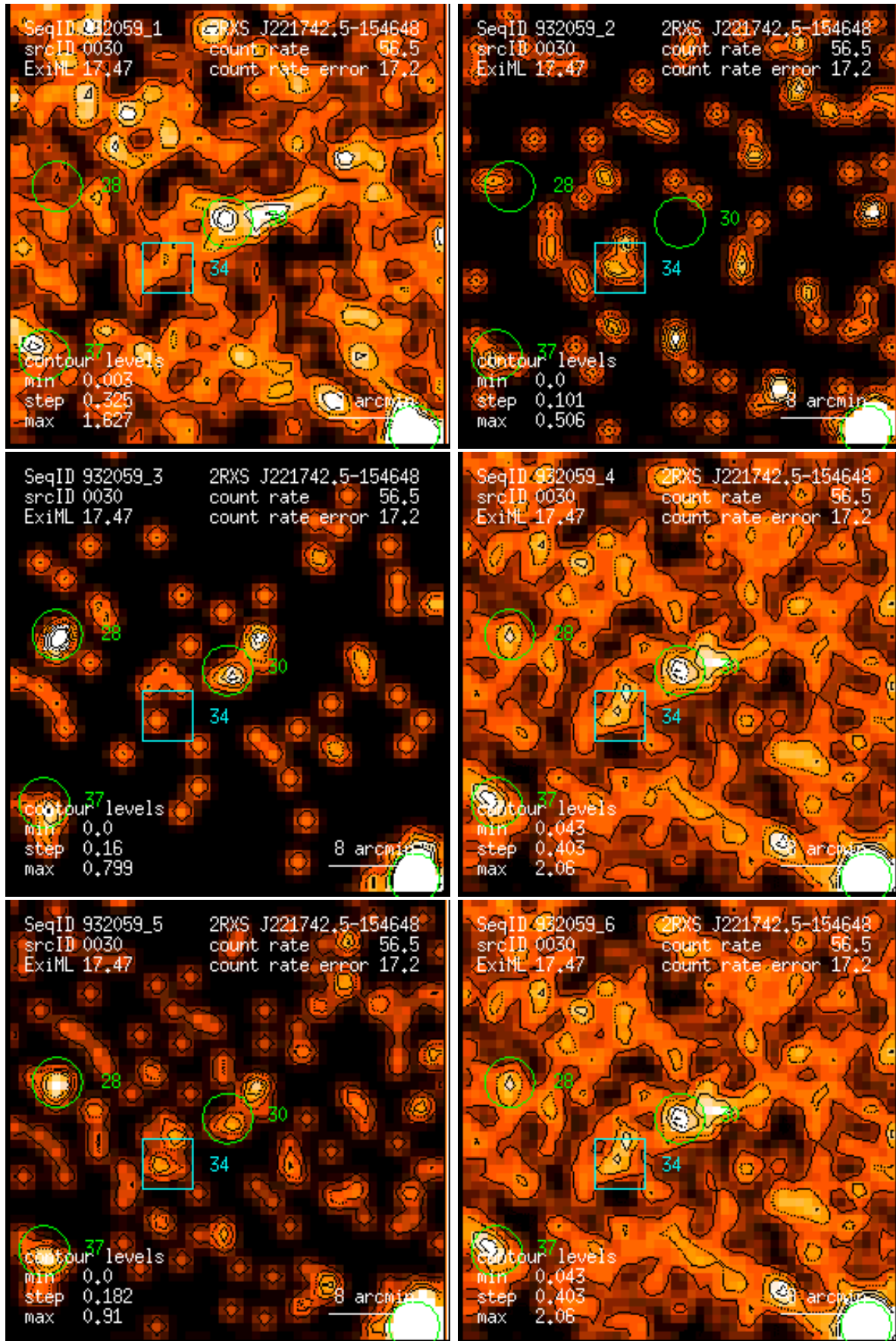
Figure 30: RASS 932059: detection 0030: band rate images, Gaussian filter: (1) PSPC channels 11 – 41, (2) 52 – 90, (3) 91 – 201, (4) 11 – 235, (5) 52 – 201, (6) 11 – 201. Broad band rates in counts/ks. Band rate contour levels in counts/ks/arcmin 2 .
