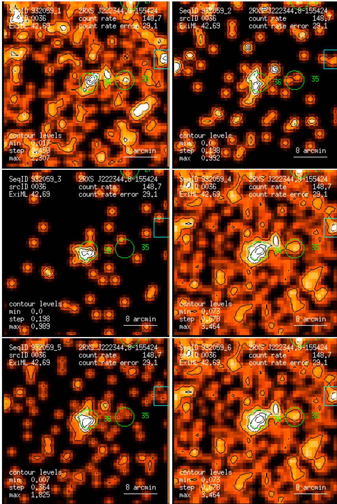
Figure 36: RASS 932059: detection 0036: band rate images, Gaussian filter: (1) PSPC channels 11 – 41, (2) 52 – 90, (3) 91 – 201, (4) 11 – 235, (5) 52 – 201, (6) 11 – 201. Broad band rates in counts/ks. Band rate contour levels in counts/ks/arcmin 2 .
