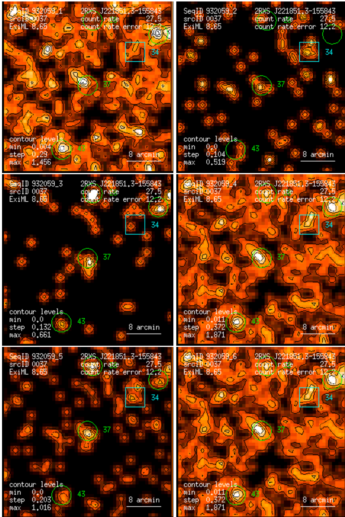
Figure 37: RASS 932059: detection 0037: band rate images, Gaussian filter: (1) PSPC channels 11 – 41, (2) 52 – 90, (3) 91 – 201, (4) 11 – 235, (5) 52 – 201, (6) 11 – 201. Broad band rates in counts/ks. Band rate contour levels in counts/ks/arcmin 2 .
