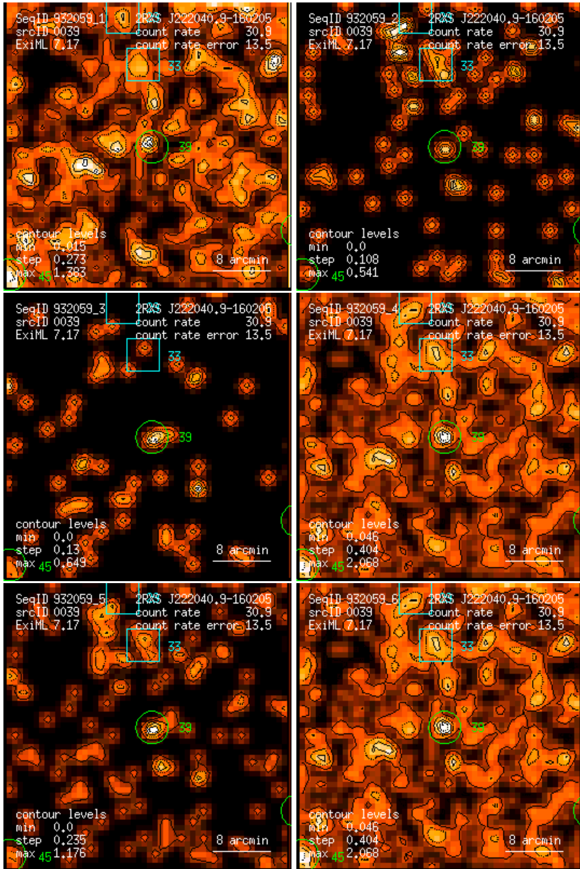
Figure 39: RASS 932059: detection 0039: band rate images, Gaussian filter: (1) PSPC channels 11 – 41, (2) 52 – 90, (3) 91 – 201, (4) 11 – 235, (5) 52 – 201, (6) 11 – 201. Broad band rates in counts/ks. Band rate contour levels in counts/ks/arcmin 2 .
