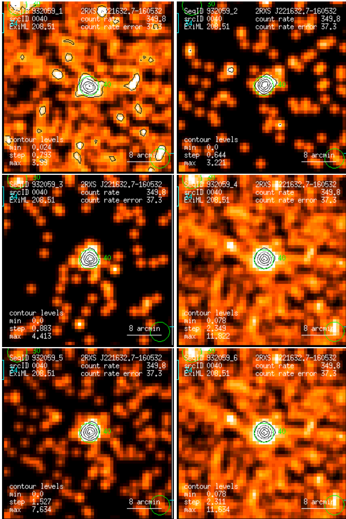
Figure 40: RASS 932059: detection 0040: band rate images, Gaussian filter: (1) PSPC channels 11 – 41, (2) 52 – 90, (3) 91 – 201, (4) 11 – 235, (5) 52 – 201, (6) 11 – 201. Broad band rates in counts/ks. Band rate contour levels in counts/ks/arcmin 2 .
