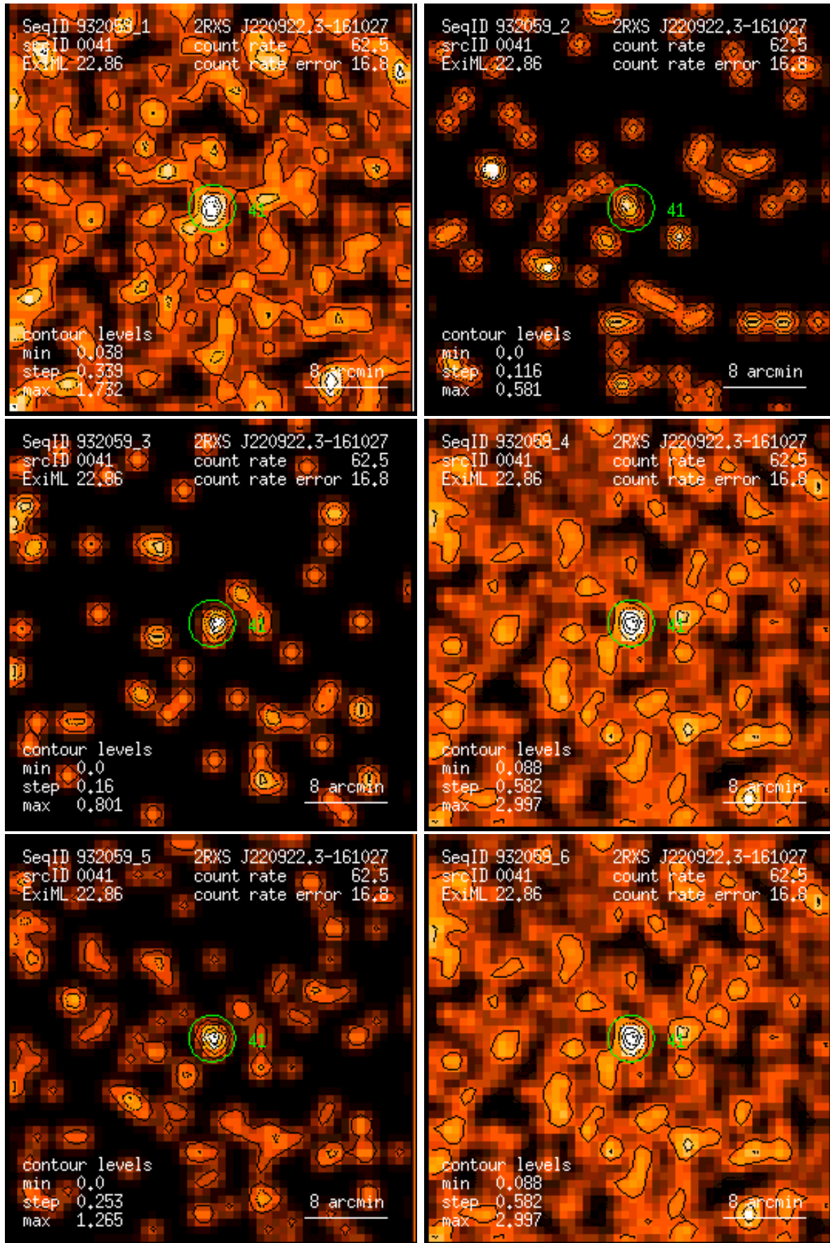
Figure 41: RASS 932059: detection 0041: band rate images, Gaussian filter: (1) PSPC channels 11 – 41, (2) 52 – 90, (3) 91 – 201, (4) 11 – 235, (5) 52 – 201, (6) 11 – 201. Broad band rates in counts/ks. Band rate contour levels in counts/ks/arcmin 2 .
