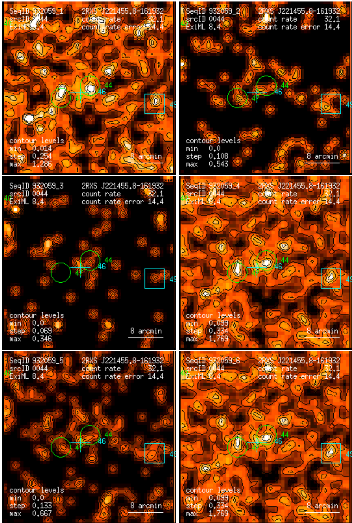
Figure 44: RASS 932059: detection 0044: band rate images, Gaussian filter: (1) PSPC channels 11 – 41, (2) 52 – 90, (3) 91 – 201, (4) 11 – 235, (5) 52 – 201, (6) 11 – 201. Broad band rates in counts/ks. Band rate contour levels in counts/ks/arcmin 2 .
