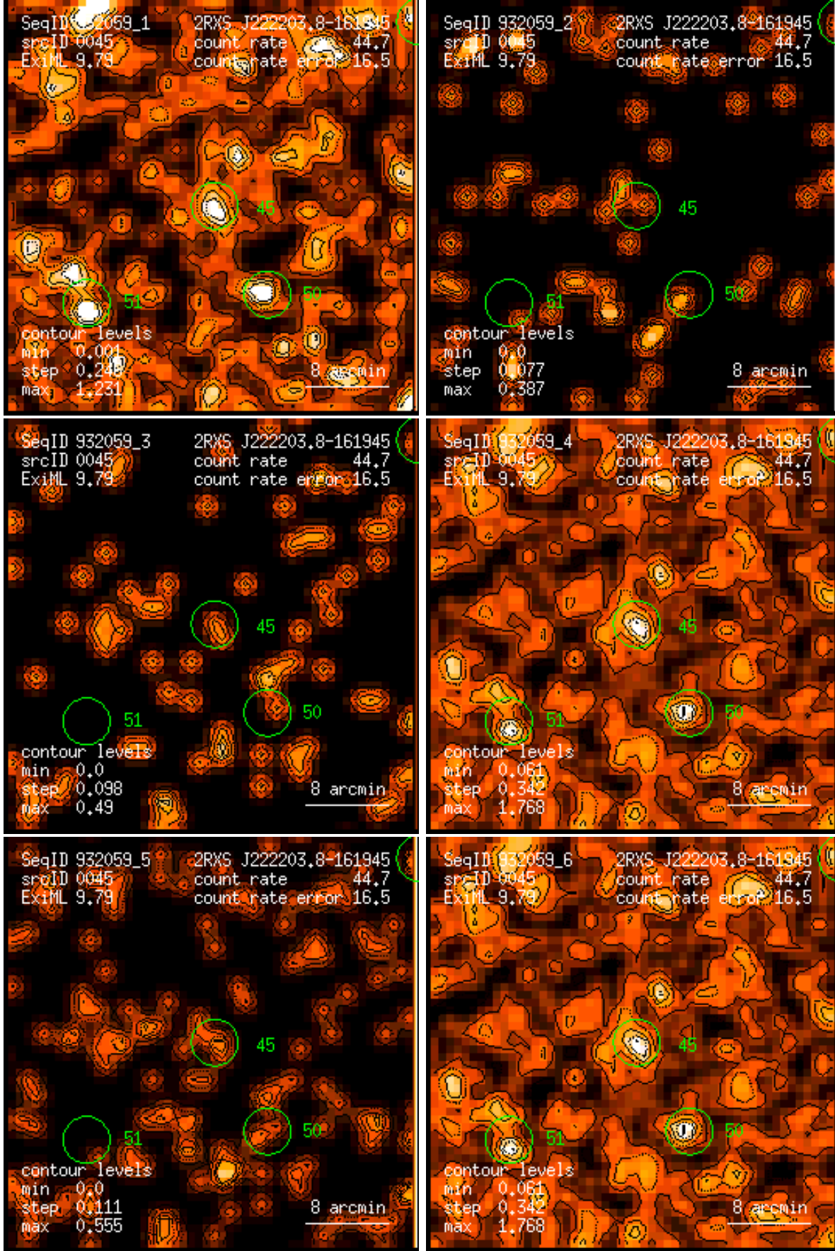
Figure 45: RASS 932059: detection 0045: band rate images, Gaussian filter: (1) PSPC channels 11 – 41, (2) 52 – 90, (3) 91 – 201, (4) 11 – 235, (5) 52 – 201, (6) 11 – 201. Broad band rates in counts/ks. Band rate contour levels in counts/ks/arcmin 2 .
