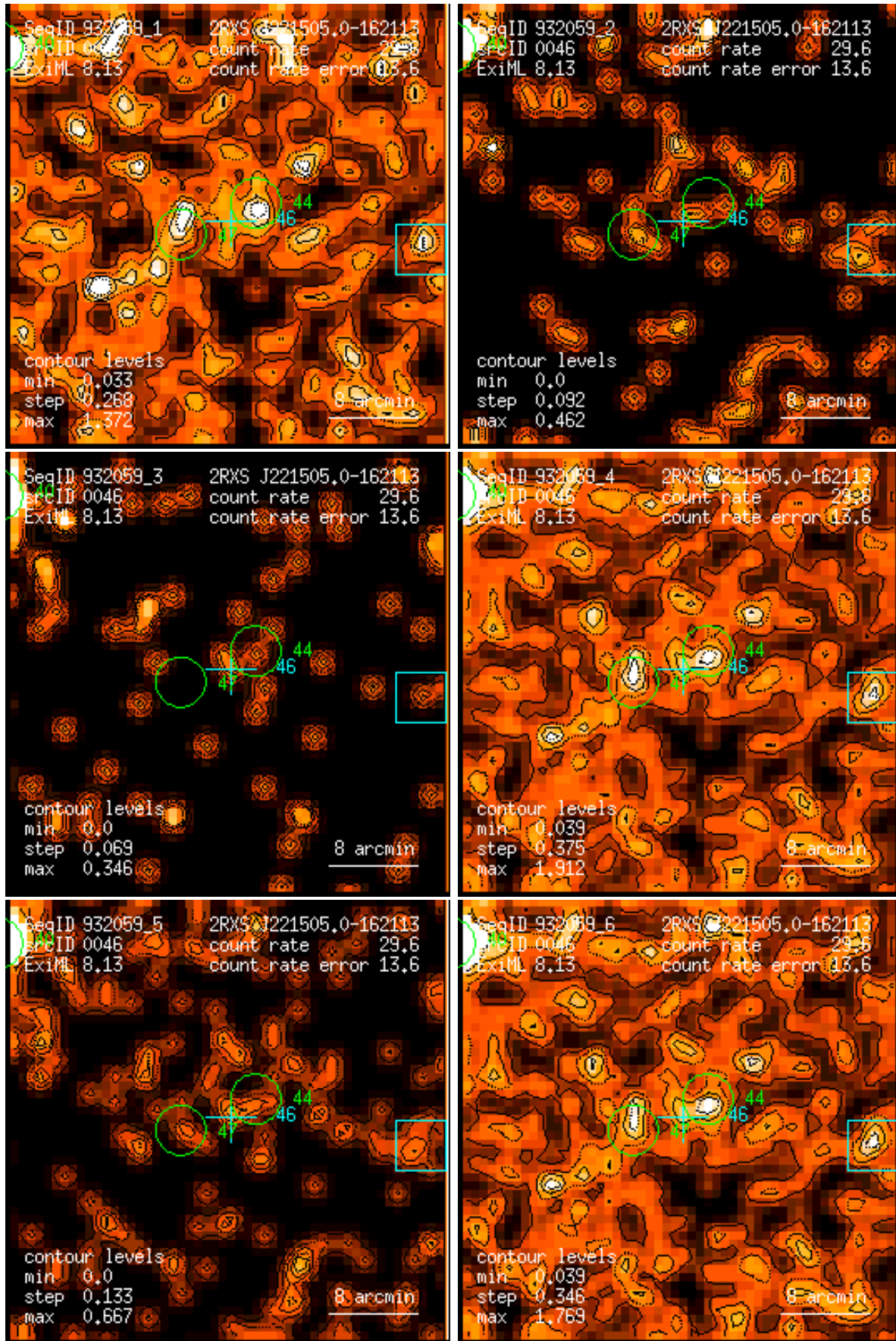
Figure 46: RASS 932059: detection 0046: band rate images, Gaussian filter: (1) PSPC channels 11 – 41, (2) 52 – 90, (3) 91 – 201, (4) 11 – 235, (5) 52 – 201, (6) 11 – 201. Broad band rates in counts/ks. Band rate contour levels in counts/ks/arcmin 2 .
