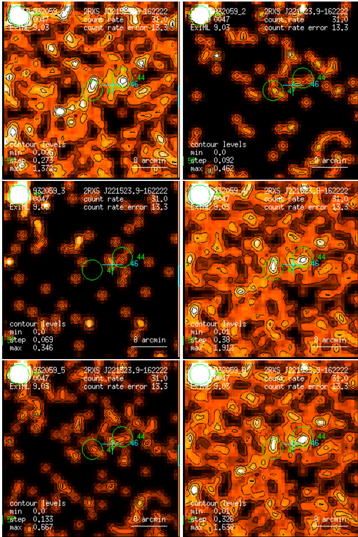
Figure 47: RASS 932059: detection 0047: band rate images, Gaussian filter: (1) PSPC channels 11 – 41, (2) 52 – 90, (3) 91 – 201, (4) 11 – 235, (5) 52 – 201, (6) 11 – 201. Broad band rates in counts/ks. Band rate contour levels in counts/ks/arcmin 2 .
