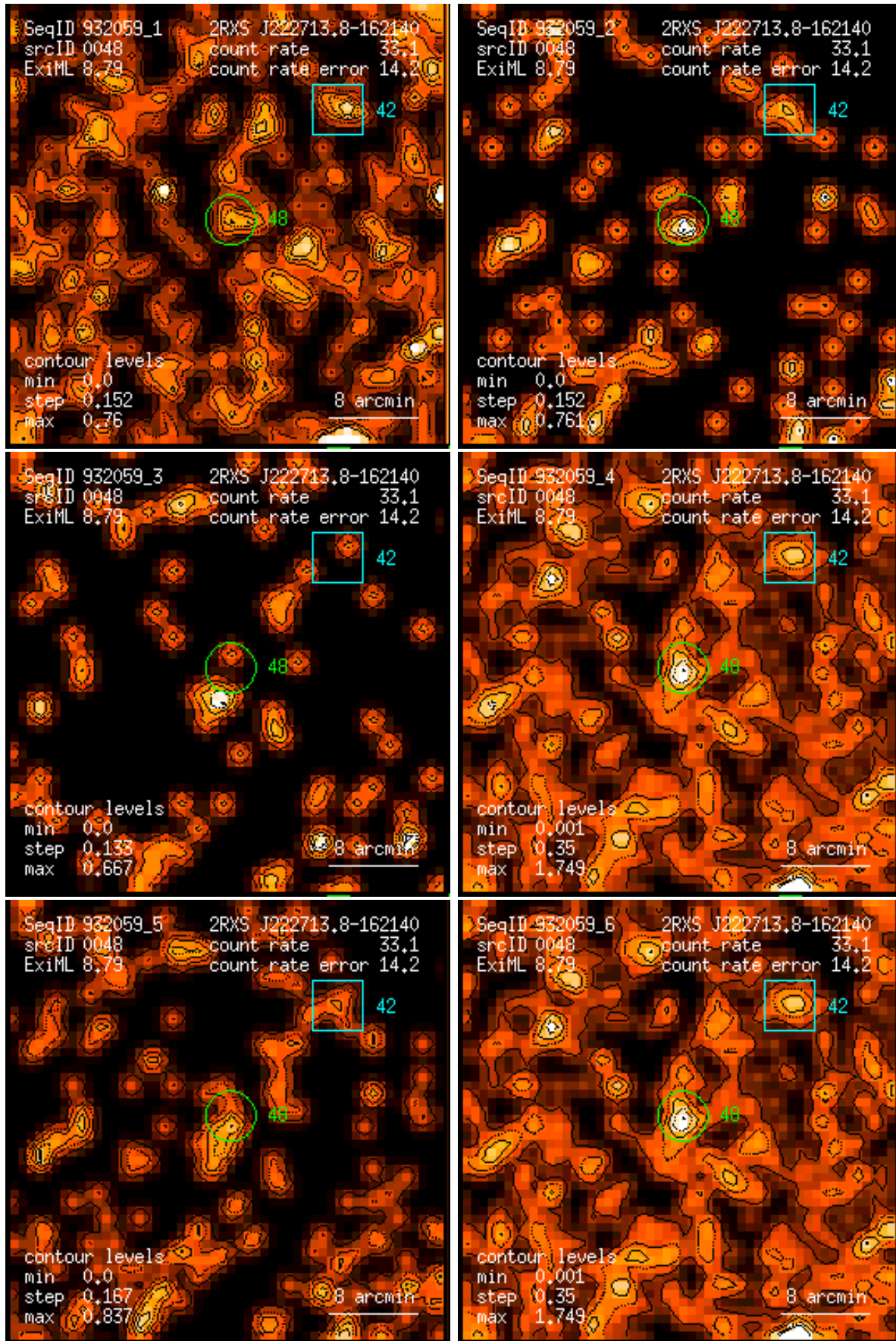
Figure 48: RASS 932059: detection 0048: band rate images, Gaussian filter: (1) PSPC channels 11 – 41, (2) 52 – 90, (3) 91 – 201, (4) 11 – 235, (5) 52 – 201, (6) 11 – 201. Broad band rates in counts/ks. Band rate contour levels in counts/ks/arcmin 2 .
