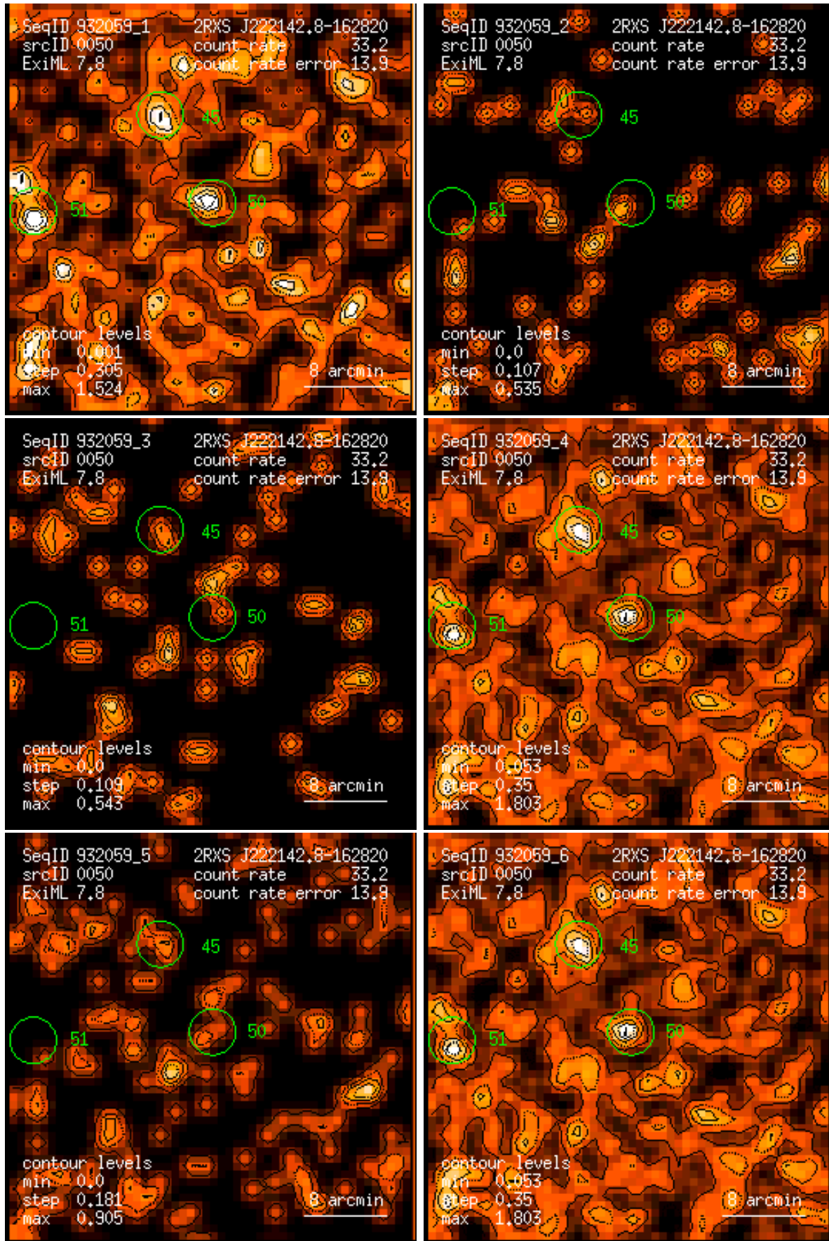
Figure 50: RASS 932059: detection 0050: band rate images, Gaussian filter: (1) PSPC channels 11 – 41, (2) 52 – 90, (3) 91 – 201, (4) 11 – 235, (5) 52 – 201, (6) 11 – 201. Broad band rates in counts/ks. Band rate contour levels in counts/ks/arcmin 2 .
