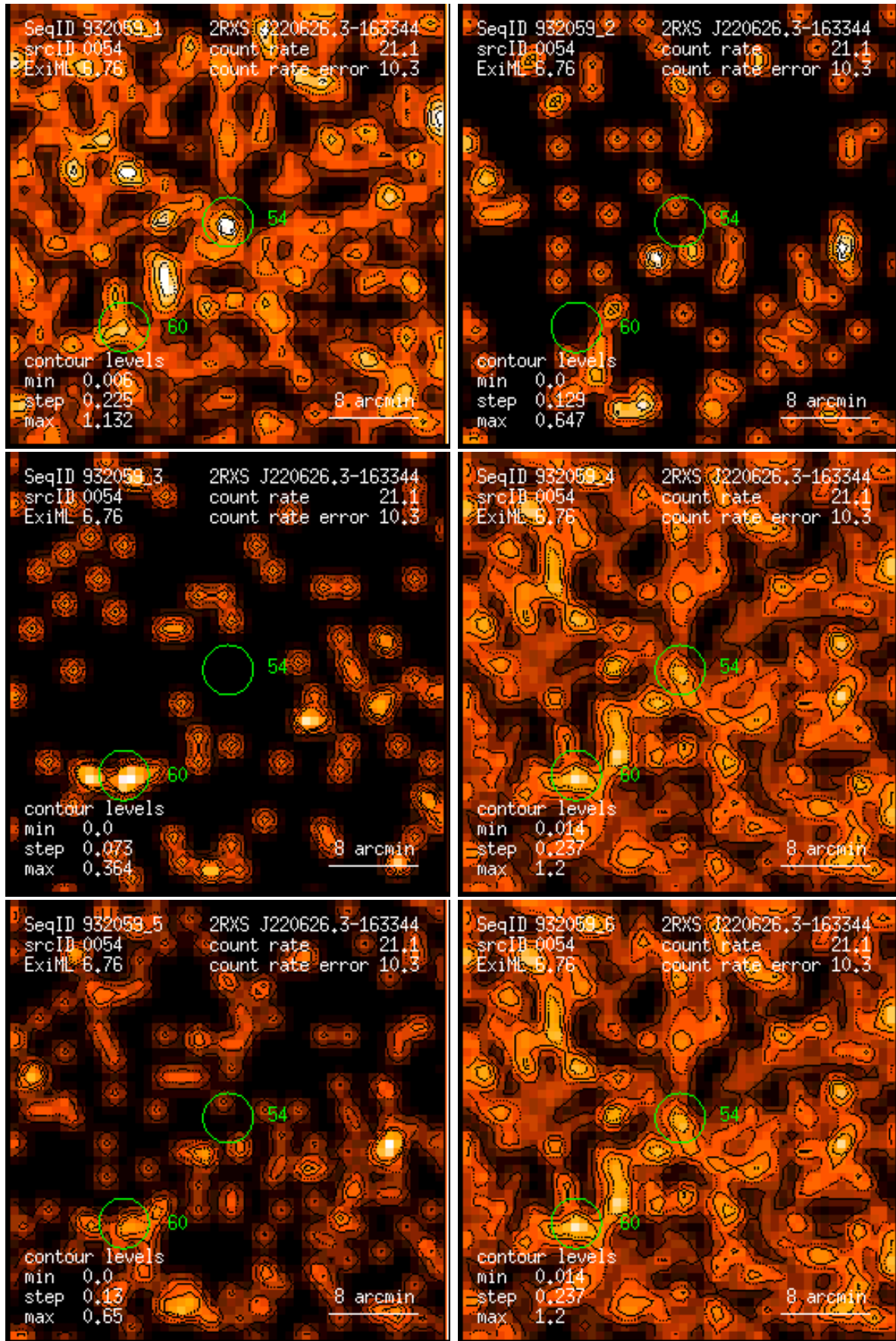
Figure 54: RASS 932059: detection 0054: band rate images, Gaussian filter: (1) PSPC channels 11 – 41, (2) 52 – 90, (3) 91 – 201, (4) 11 – 235, (5) 52 – 201, (6) 11 – 201. Broad band rates in counts/ks. Band rate contour levels in counts/ks/arcmin 2 .
