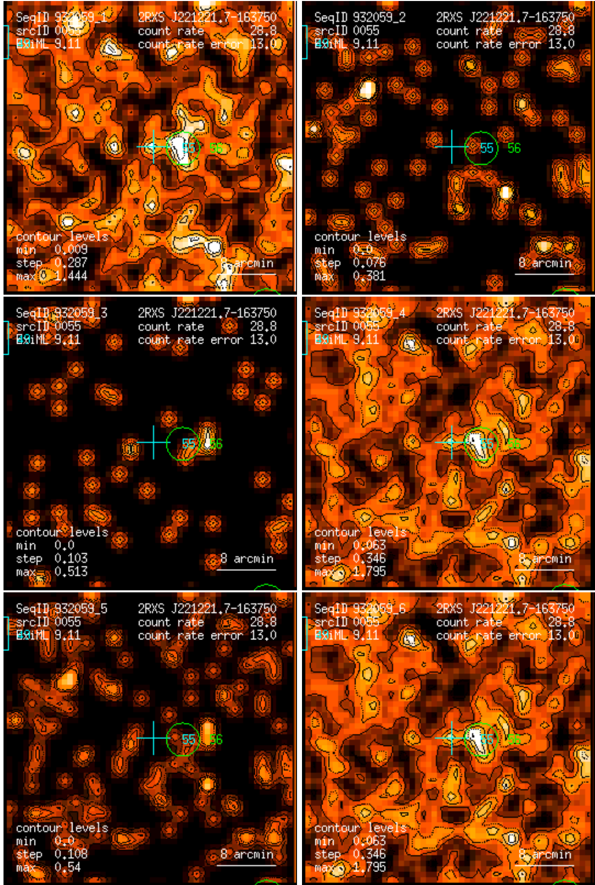
Figure 55: RASS 932059: detection 0055: band rate images, Gaussian filter: (1) PSPC channels 11 – 41, (2) 52 – 90, (3) 91 – 201, (4) 11 – 235, (5) 52 – 201, (6) 11 – 201. Broad band rates in counts/ks. Band rate contour levels in counts/ks/arcmin 2 .
