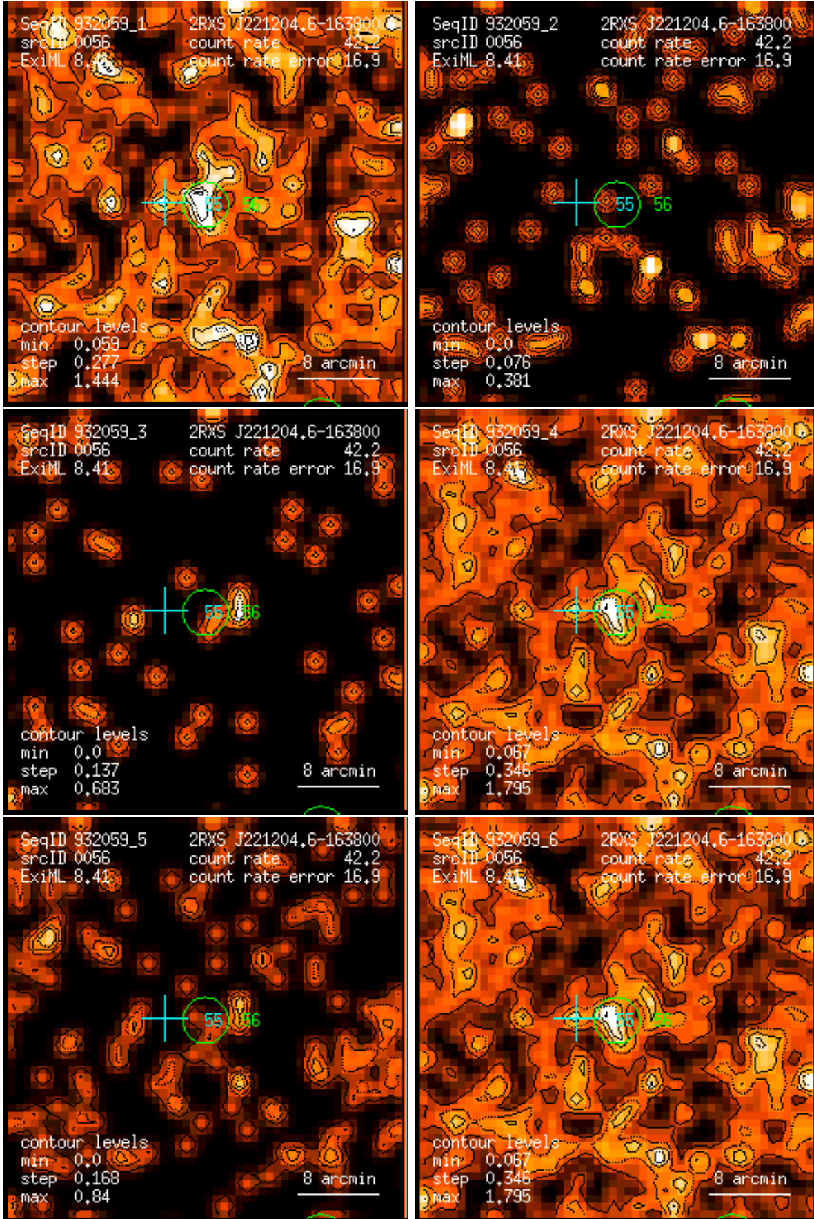
Figure 56: RASS 932059: detection 0056: band rate images, Gaussian filter: (1) PSPC channels 11 – 41, (2) 52 – 90, (3) 91 – 201, (4) 11 – 235, (5) 52 – 201, (6) 11 – 201. Broad band rates in counts/ks. Band rate contour levels in counts/ks/arcmin 2 .
