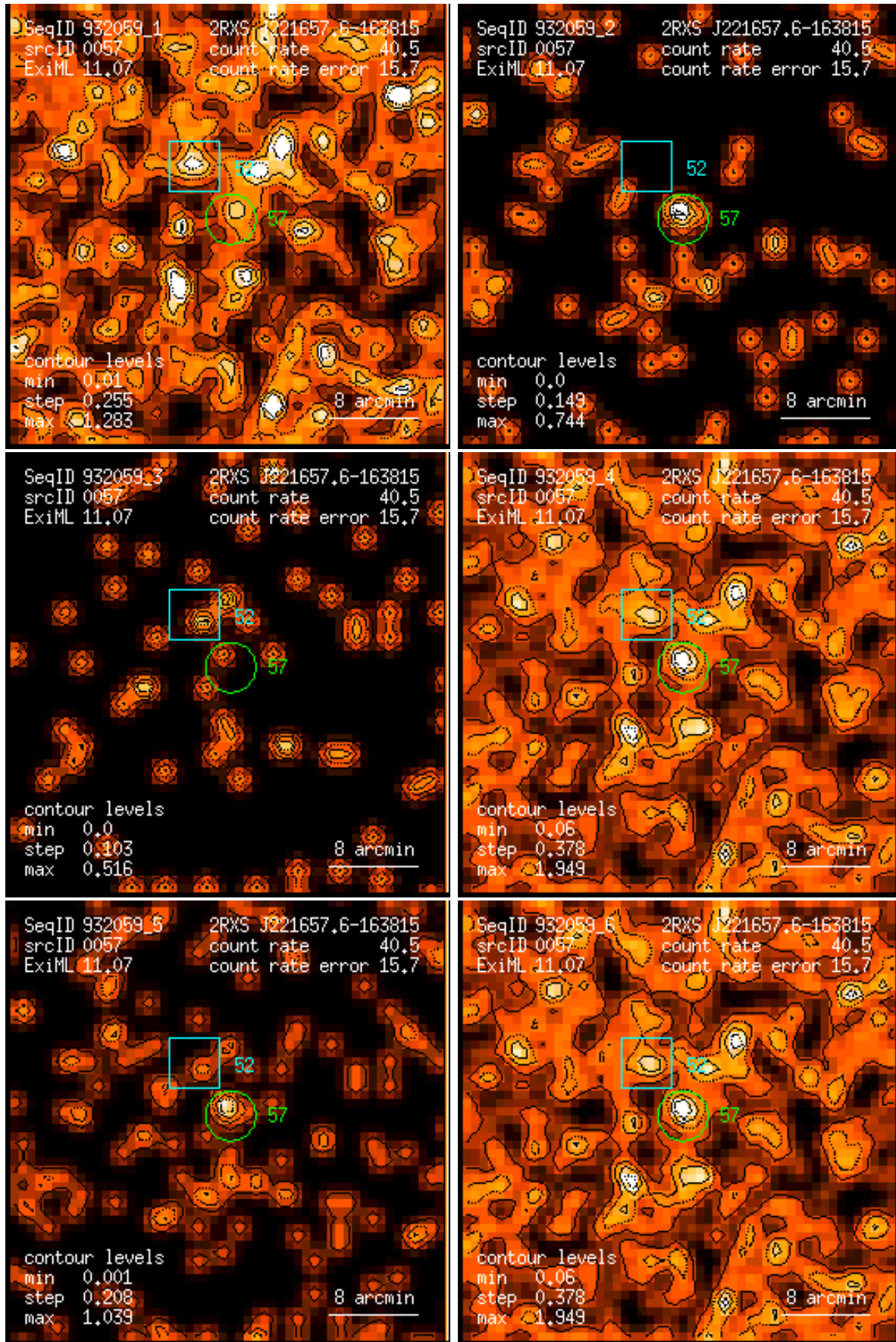
Figure 57: RASS 932059: detection 0057: band rate images, Gaussian filter: (1) PSPC channels 11 – 41, (2) 52 – 90, (3) 91 – 201, (4) 11 – 235, (5) 52 – 201, (6) 11 – 201. Broad band rates in counts/ks. Band rate contour levels in counts/ks/arcmin 2 .
