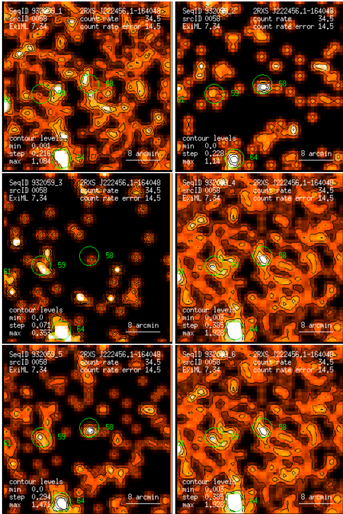
Figure 58: RASS 932059: detection 0058: band rate images, Gaussian filter: (1) PSPC channels 11 – 41, (2) 52 – 90, (3) 91 – 201, (4) 11 – 235, (5) 52 – 201, (6) 11 – 201. Broad band rates in counts/ks. Band rate contour levels in counts/ks/arcmin 2 .
