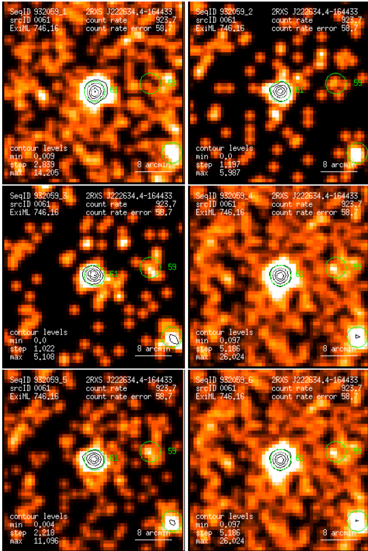
Figure 61: RASS 932059: detection 0061: band rate images, Gaussian filter: (1) PSPC channels 11 – 41, (2) 52 – 90, (3) 91 – 201, (4) 11 – 235, (5) 52 – 201, (6) 11 – 201. Broad band rates in counts/ks. Band rate contour levels in counts/ks/arcmin 2 .
