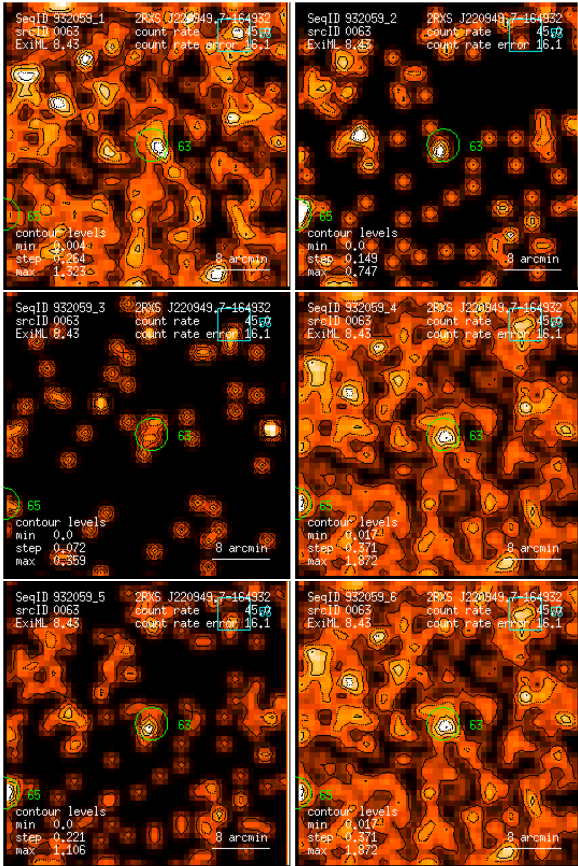
Figure 63: RASS 932059: detection 0063: band rate images, Gaussian filter: (1) PSPC channels 11 – 41, (2) 52 – 90, (3) 91 – 201, (4) 11 – 235, (5) 52 – 201, (6) 11 – 201. Broad band rates in counts/ks. Band rate contour levels in counts/ks/arcmin 2 .
