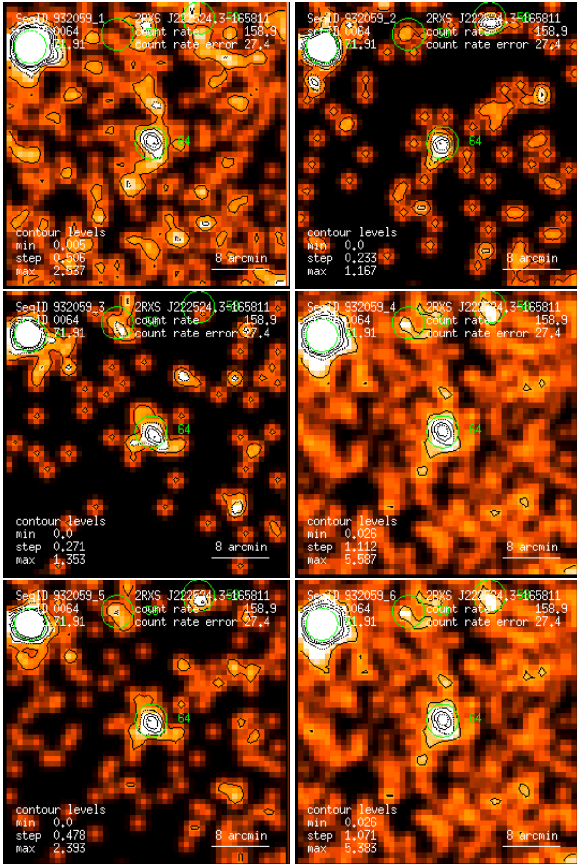
Figure 64: RASS 932059: detection 0064: band rate images, Gaussian filter: (1) PSPC channels 11 – 41, (2) 52 – 90, (3) 91 – 201, (4) 11 – 235, (5) 52 – 201, (6) 11 – 201. Broad band rates in counts/ks. Band rate contour levels in counts/ks/arcmin 2 .
