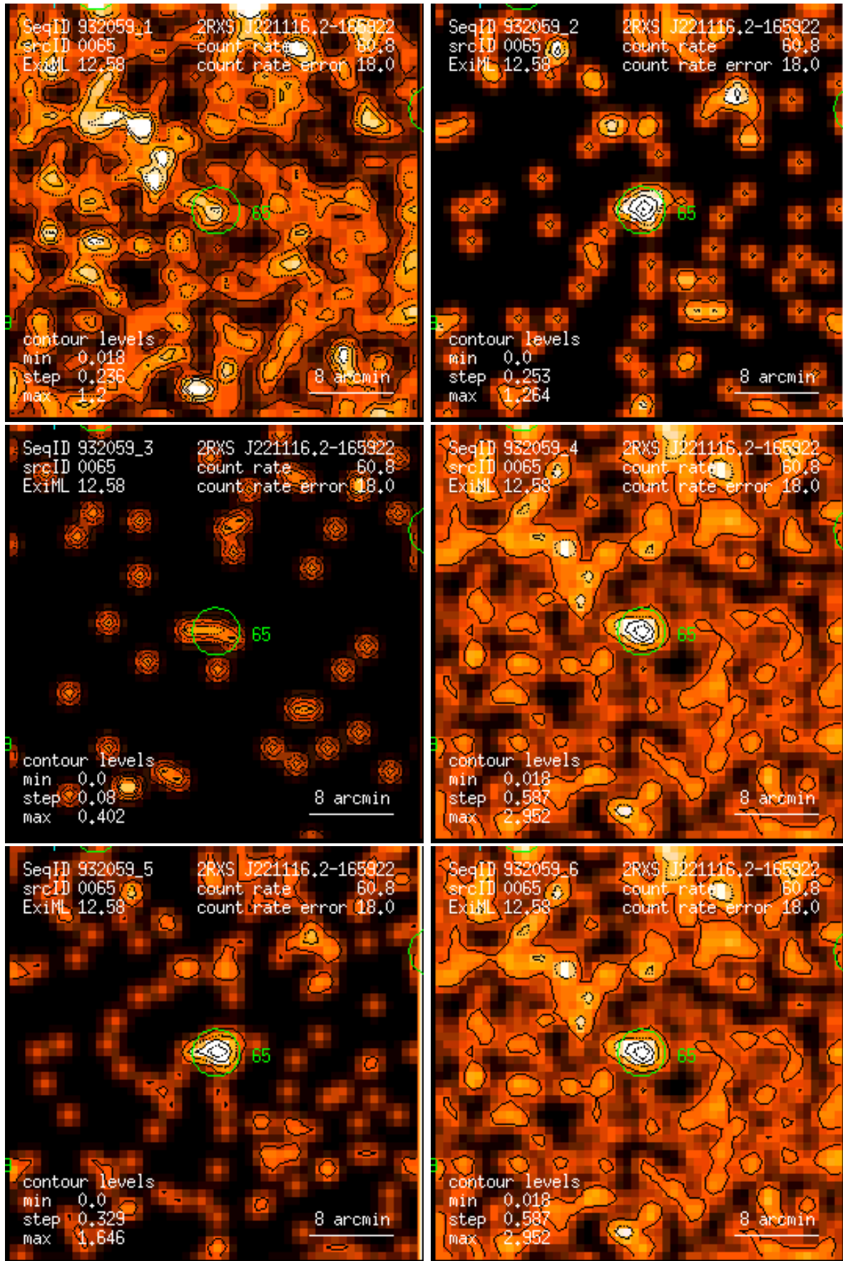
Figure 65: RASS 932059: detection 0065: band rate images, Gaussian filter: (1) PSPC channels 11 – 41, (2) 52 – 90, (3) 91 – 201, (4) 11 – 235, (5) 52 – 201, (6) 11 – 201. Broad band rates in counts/ks. Band rate contour levels in counts/ks/arcmin 2 .
