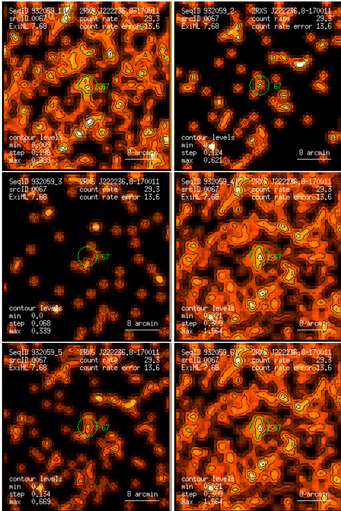
Figure 67: RASS 932059: detection 0067: band rate images, Gaussian filter: (1) PSPC channels 11 – 41, (2) 52 – 90, (3) 91 – 201, (4) 11 – 235, (5) 52 – 201, (6) 11 – 201. Broad band rates in counts/ks. Band rate contour levels in counts/ks/arcmin 2 .
