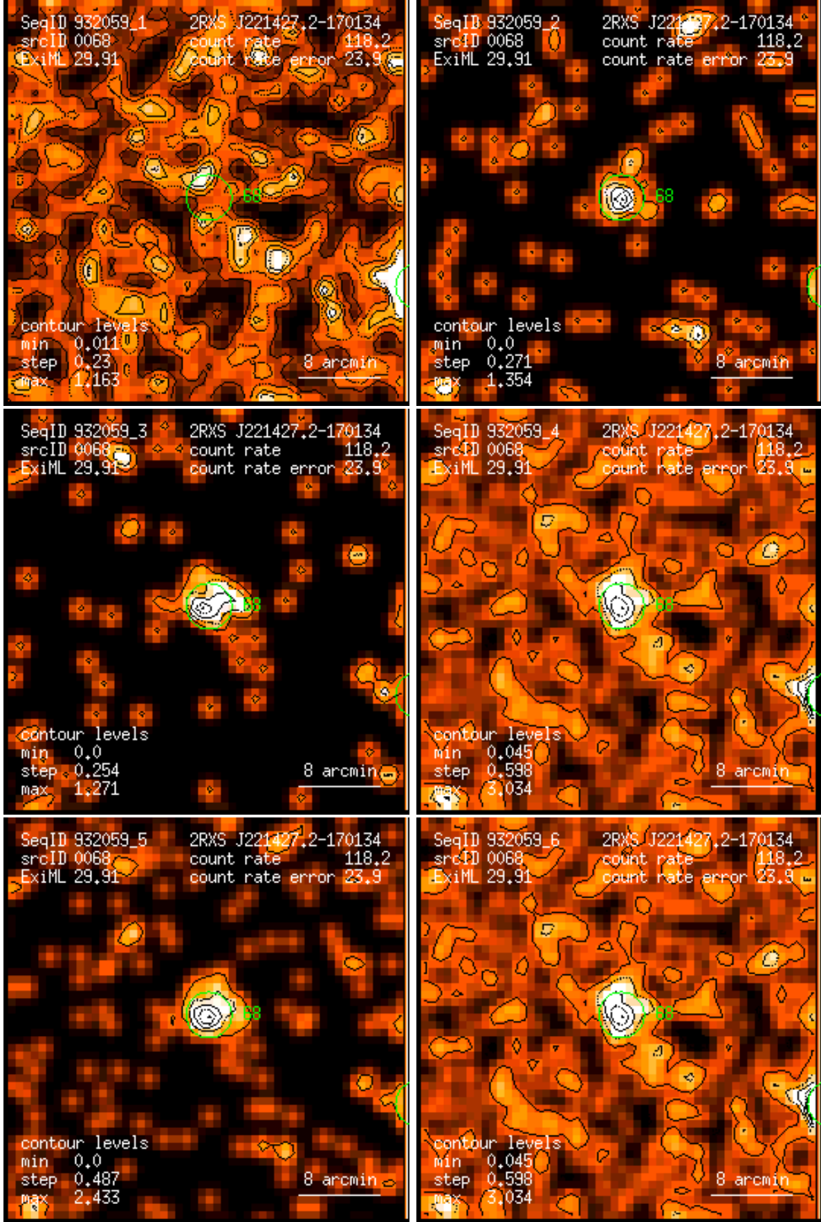
Figure 68: RASS 932059: detection 0068: band rate images, Gaussian filter: (1) PSPC channels 11 – 41, (2) 52 – 90, (3) 91 – 201, (4) 11 – 235, (5) 52 – 201, (6) 11 – 201. Broad band rates in counts/ks. Band rate contour levels in counts/ks/arcmin 2 .
