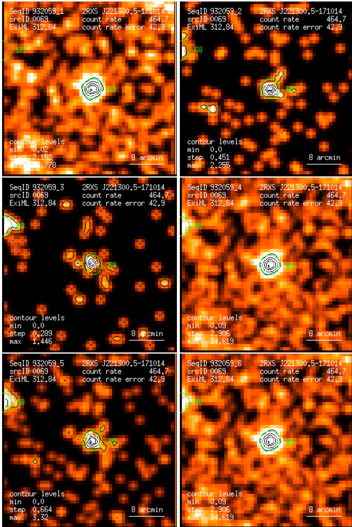
Figure 69: RASS 932059: detection 0069: band rate images, Gaussian filter: (1) PSPC channels 11 – 41, (2) 52 – 90, (3) 91 – 201, (4) 11 – 235, (5) 52 – 201, (6) 11 – 201. Broad band rates in counts/ks. Band rate contour levels in counts/ks/arcmin 2 .
