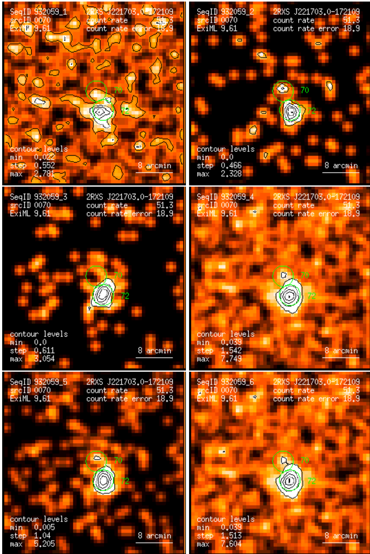
Figure 70: RASS 932059: detection 0070: band rate images, Gaussian filter: (1) PSPC channels 11 – 41, (2) 52 – 90, (3) 91 – 201, (4) 11 – 235, (5) 52 – 201, (6) 11 – 201. Broad band rates in counts/ks. Band rate contour levels in counts/ks/arcmin 2 .
