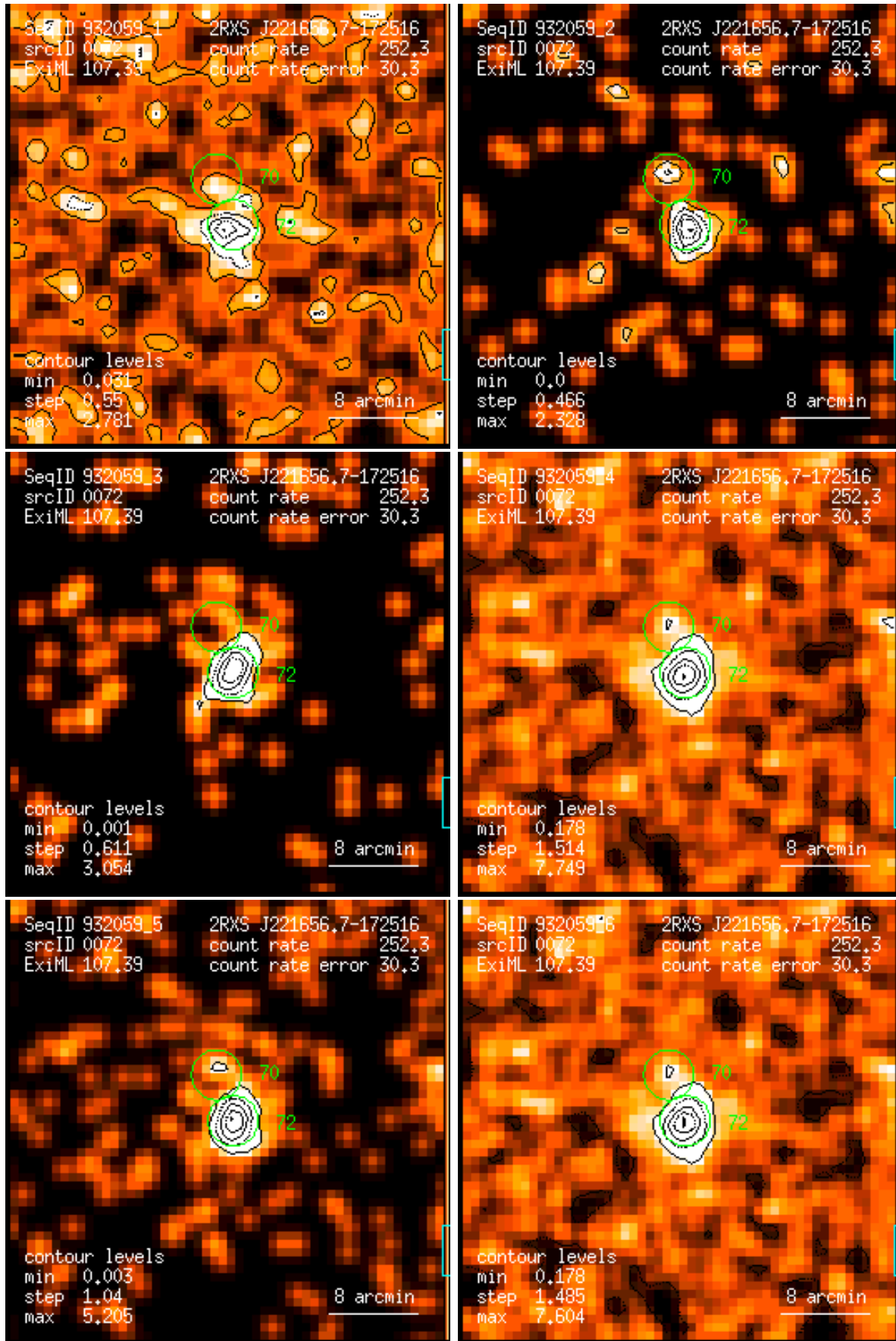
Figure 72: RASS 932059: detection 0072: band rate images, Gaussian filter: (1) PSPC channels 11 – 41, (2) 52 – 90, (3) 91 – 201, (4) 11 – 235, (5) 52 – 201, (6) 11 – 201. Broad band rates in counts/ks. Band rate contour levels in counts/ks/arcmin 2 .
