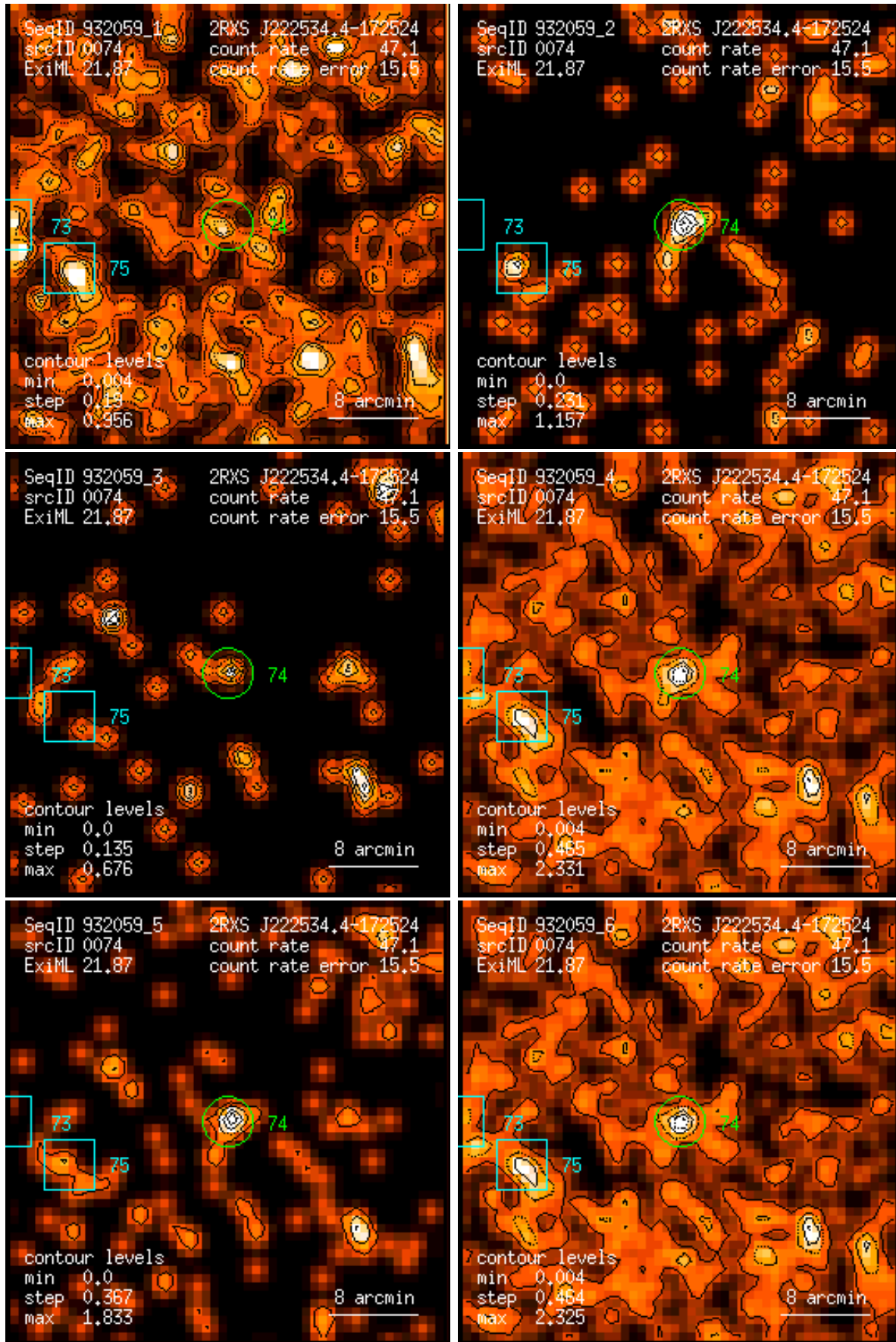
Figure 74: RASS 932059: detection 0074: band rate images, Gaussian filter: (1) PSPC channels 11 – 41, (2) 52 – 90, (3) 91 – 201, (4) 11 – 235, (5) 52 – 201, (6) 11 – 201. Broad band rates in counts/ks. Band rate contour levels in counts/ks/arcmin 2 .
