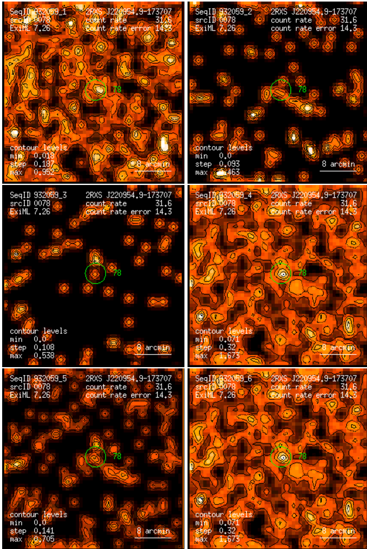
Figure 78: RASS 932059: detection 0078: band rate images, Gaussian filter: (1) PSPC channels 11 – 41, (2) 52 – 90, (3) 91 – 201, (4) 11 – 235, (5) 52 – 201, (6) 11 – 201. Broad band rates in counts/ks. Band rate contour levels in counts/ks/arcmin 2 .
