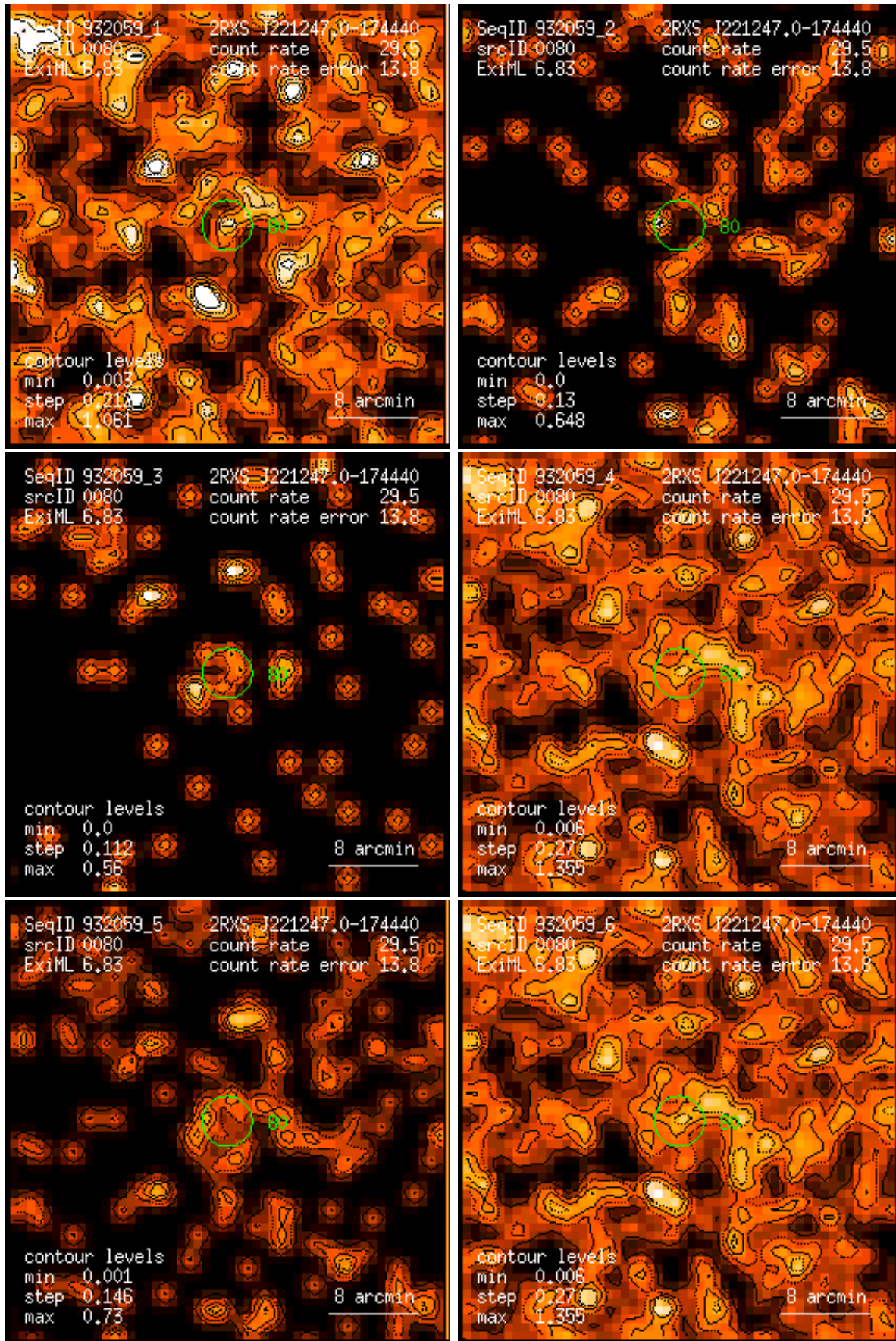
Figure 80: RASS 932059: detection 0080: band rate images, Gaussian filter: (1) PSPC channels 11 – 41, (2) 52 – 90, (3) 91 – 201, (4) 11 – 235, (5) 52 – 201, (6) 11 – 201. Broad band rates in counts/ks. Band rate contour levels in counts/ks/arcmin 2 .
