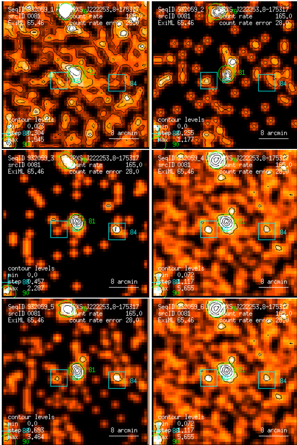
Figure 81: RASS 932059: detection 0081: band rate images, Gaussian filter: (1) PSPC channels 11 – 41, (2) 52 – 90, (3) 91 – 201, (4) 11 – 235, (5) 52 – 201, (6) 11 – 201. Broad band rates in counts/ks. Band rate contour levels in counts/ks/arcmin 2 .
