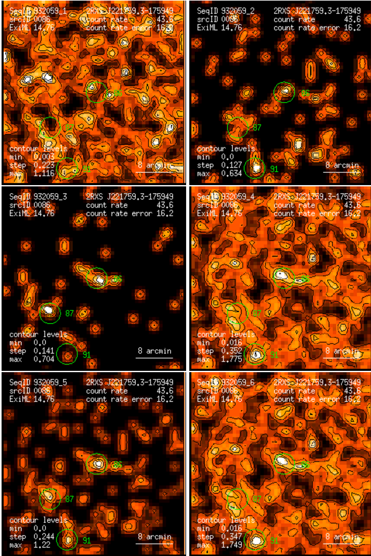
Figure 86: RASS 932059: detection 0086: band rate images, Gaussian filter: (1) PSPC channels 11 – 41, (2) 52 – 90, (3) 91 – 201, (4) 11 – 235, (5) 52 – 201, (6) 11 – 201. Broad band rates in counts/ks. Band rate contour levels in counts/ks/arcmin 2 .
