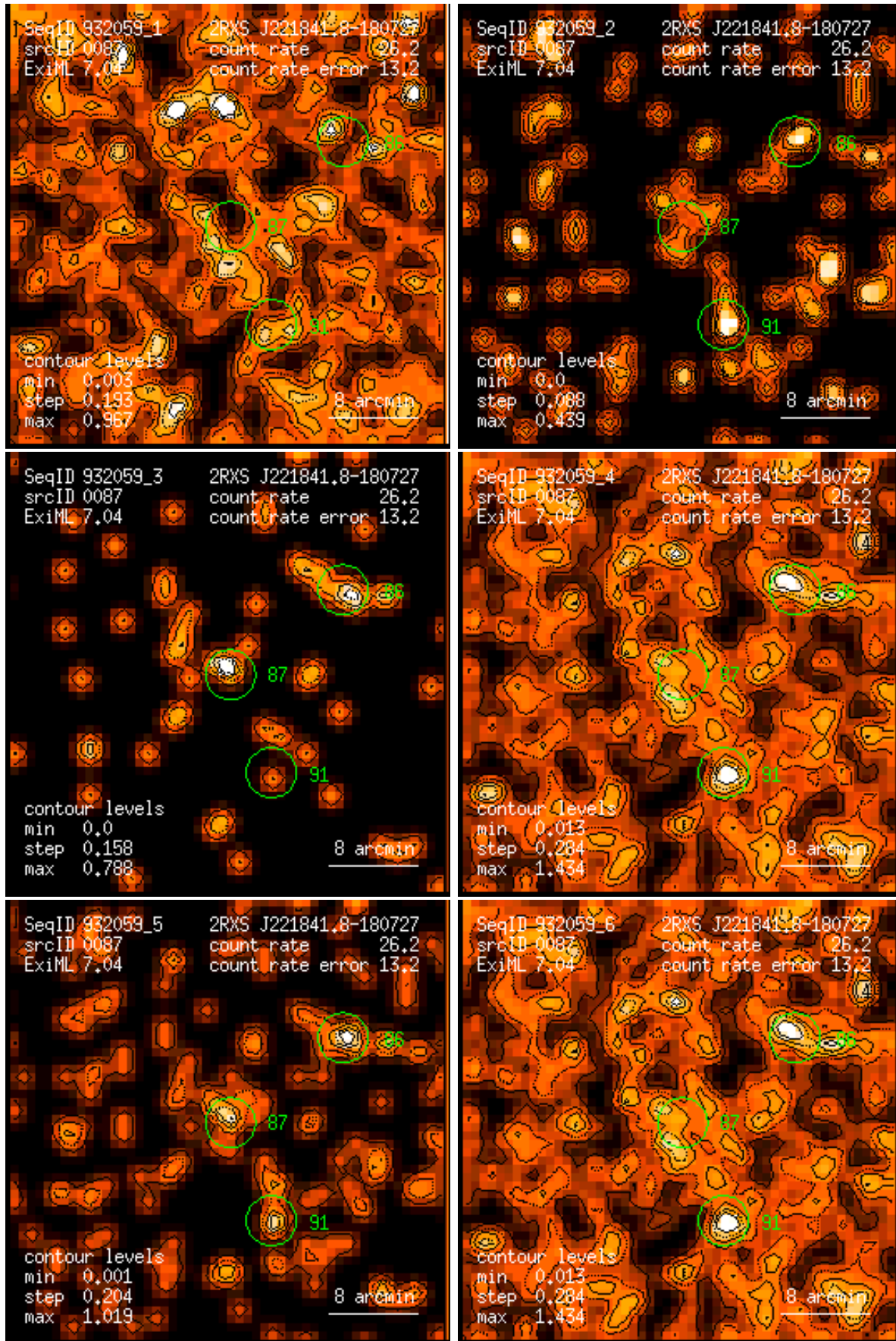
Figure 87: RASS 932059: detection 0087: band rate images, Gaussian filter: (1) PSPC channels 11 – 41, (2) 52 – 90, (3) 91 – 201, (4) 11 – 235, (5) 52 – 201, (6) 11 – 201. Broad band rates in counts/ks. Band rate contour levels in counts/ks/arcmin 2 .
