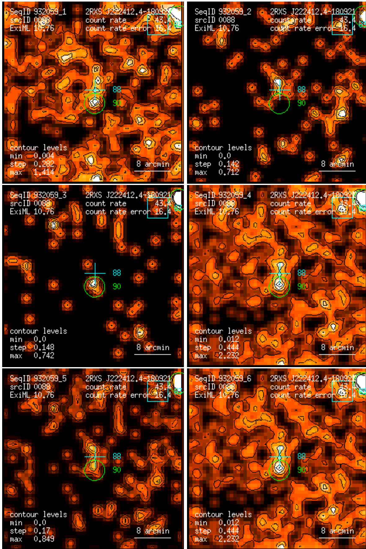
Figure 88: RASS 932059: detection 0088: band rate images, Gaussian filter: (1) PSPC channels 11 – 41, (2) 52 – 90, (3) 91 – 201, (4) 11 – 235, (5) 52 – 201, (6) 11 – 201. Broad band rates in counts/ks. Band rate contour levels in counts/ks/arcmin 2 .
