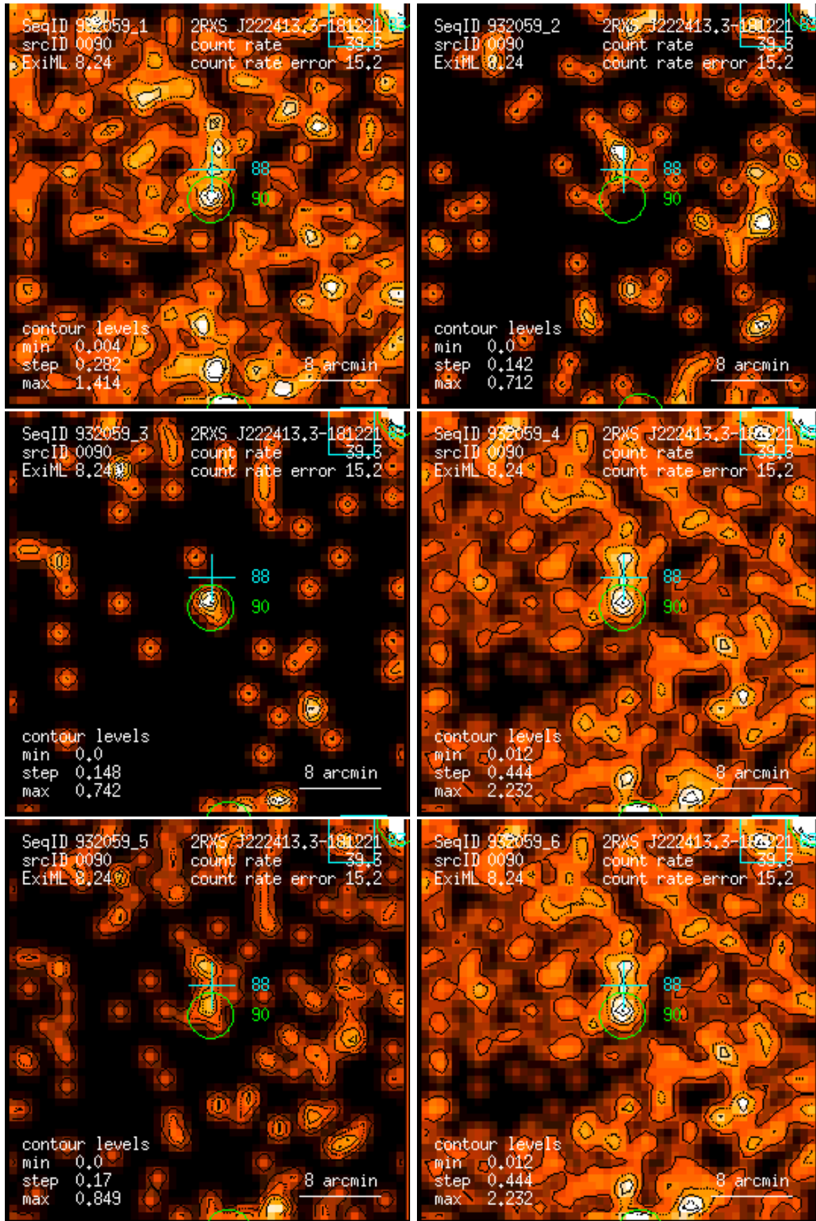
Figure 90: RASS 932059: detection 0090: band rate images, Gaussian filter: (1) PSPC channels 11 – 41, (2) 52 – 90, (3) 91 – 201, (4) 11 – 235, (5) 52 – 201, (6) 11 – 201. Broad band rates in counts/ks. Band rate contour levels in counts/ks/arcmin 2 .
