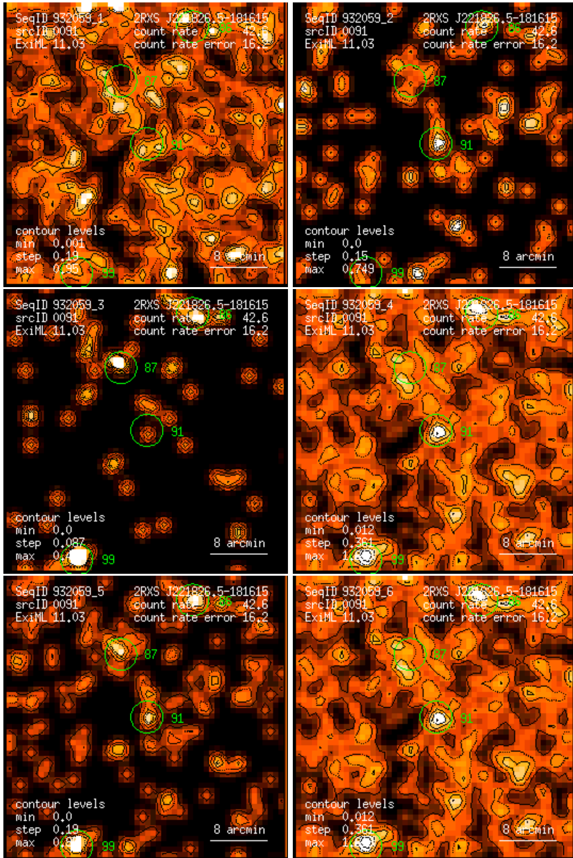
Figure 91: RASS 932059: detection 0091: band rate images, Gaussian filter: (1) PSPC channels 11 – 41, (2) 52 – 90, (3) 91 – 201, (4) 11 – 235, (5) 52 – 201, (6) 11 – 201. Broad band rates in counts/ks. Band rate contour levels in counts/ks/arcmin 2 .
