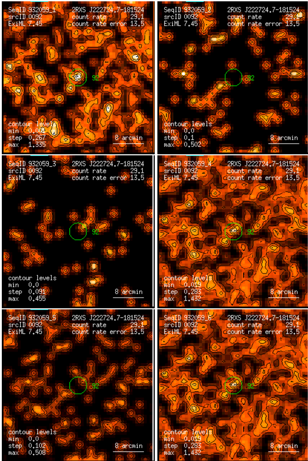
Figure 92: RASS 932059: detection 0092: band rate images, Gaussian filter: (1) PSPC channels 11 – 41, (2) 52 – 90, (3) 91 – 201, (4) 11 – 235, (5) 52 – 201, (6) 11 – 201. Broad band rates in counts/ks. Band rate contour levels in counts/ks/arcmin 2 .
