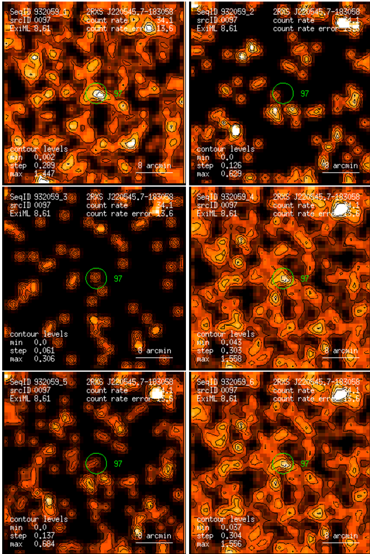
Figure 97: RASS 932059: detection 0097: band rate images, Gaussian filter: (1) PSPC channels 11 – 41, (2) 52 – 90, (3) 91 – 201, (4) 11 – 235, (5) 52 – 201, (6) 11 – 201. Broad band rates in counts/ks. Band rate contour levels in counts/ks/arcmin 2 .
