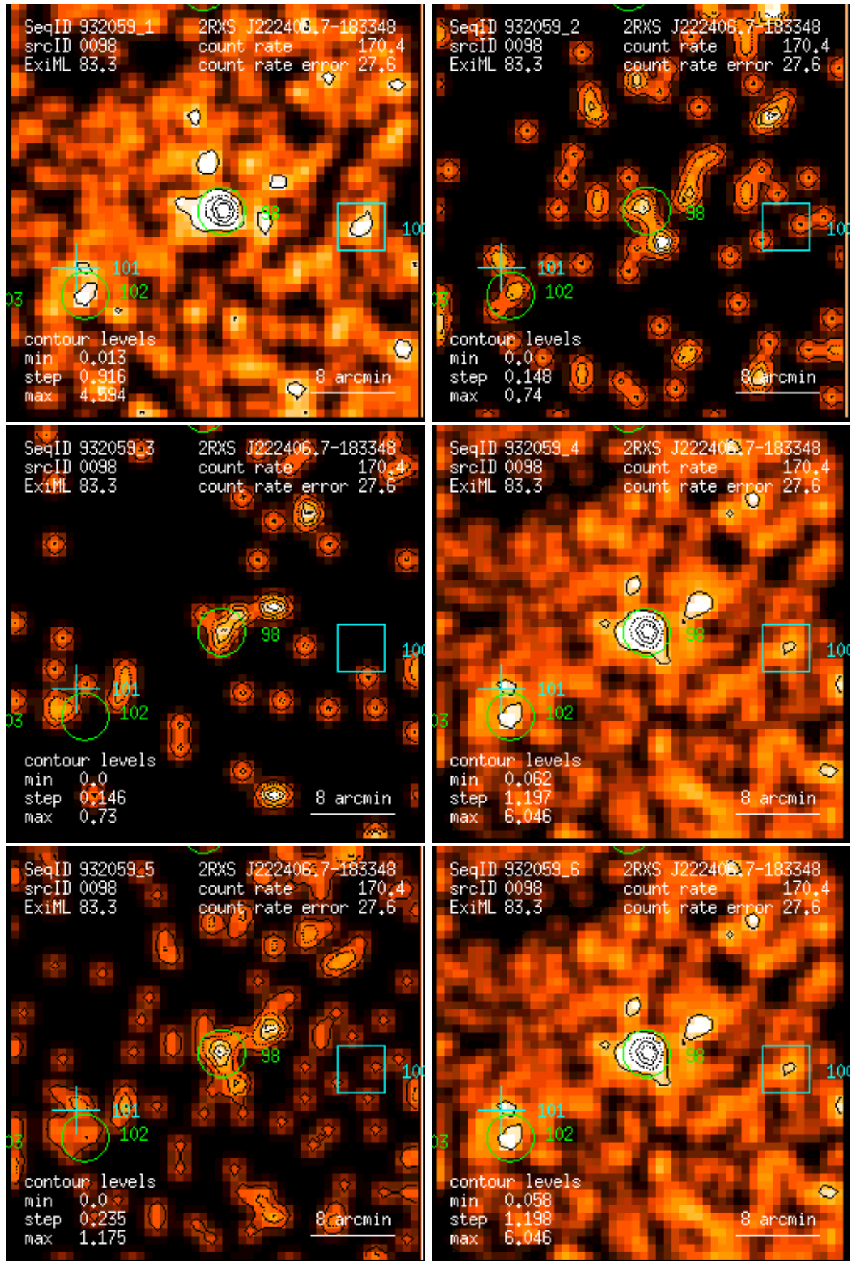
Figure 98: RASS 932059: detection 0098: band rate images, Gaussian filter: (1) PSPC channels 11 – 41, (2) 52 – 90, (3) 91 – 201, (4) 11 – 235, (5) 52 – 201, (6) 11 – 201. Broad band rates in counts/ks. Band rate contour levels in counts/ks/arcmin 2 .
