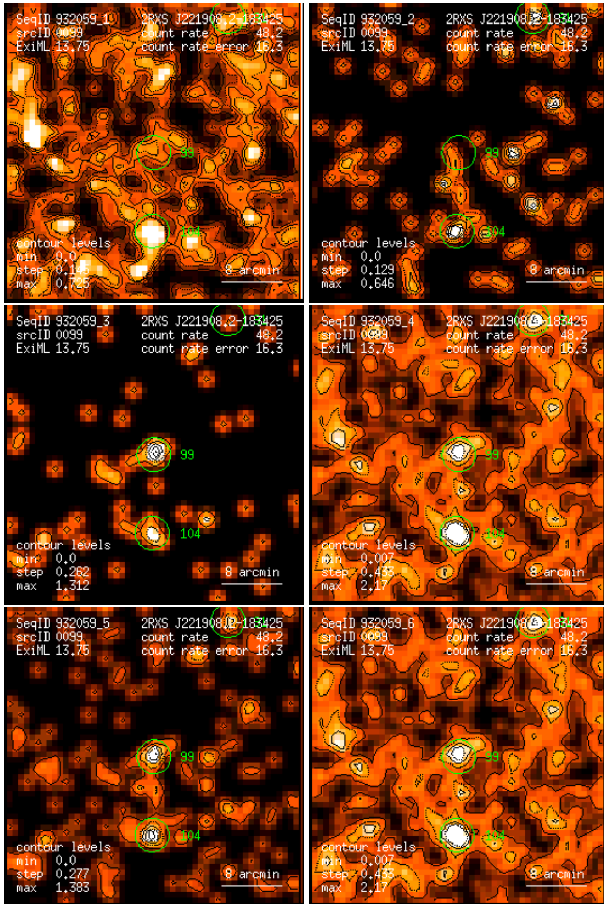
Figure 99: RASS 932059: detection 0099: band rate images, Gaussian filter: (1) PSPC channels 11 – 41, (2) 52 – 90, (3) 91 – 201, (4) 11 – 235, (5) 52 – 201, (6) 11 – 201. Broad band rates in counts/ks. Band rate contour levels in counts/ks/arcmin 2 .
