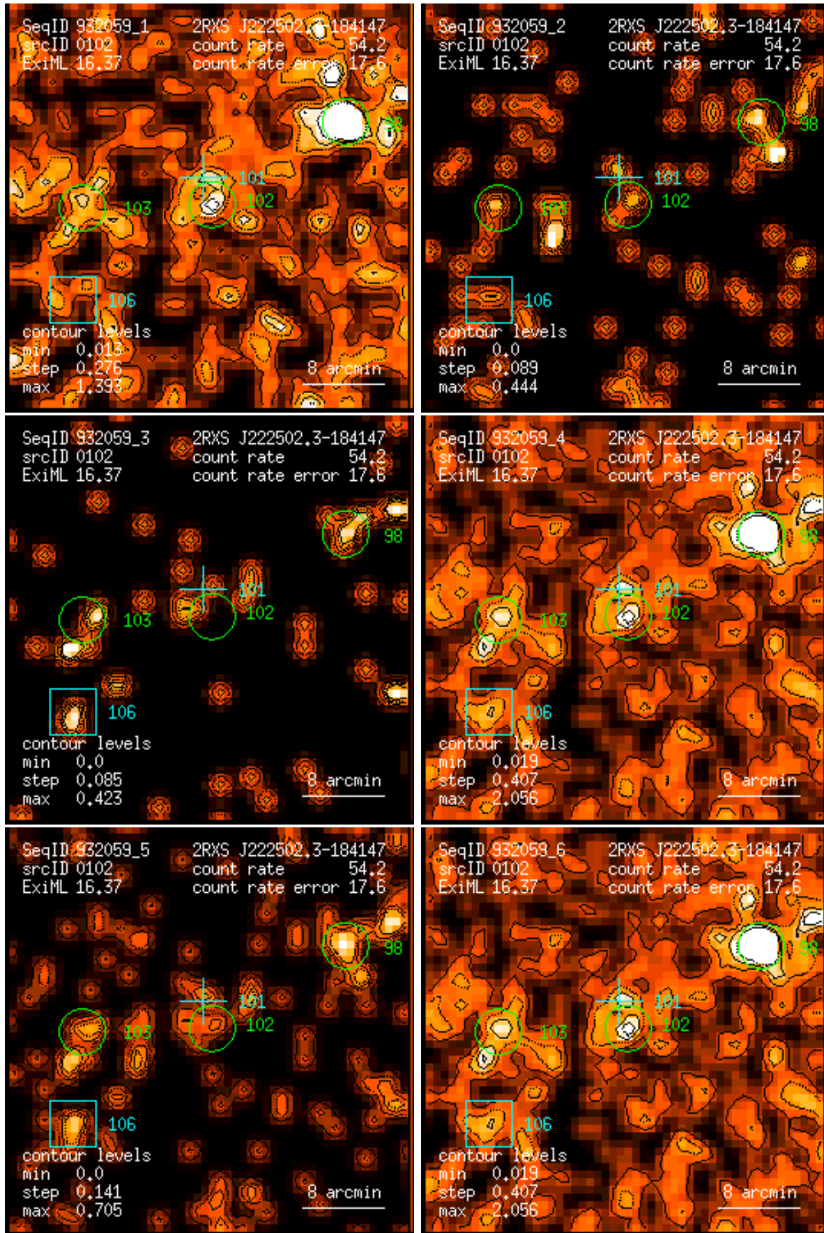
Figure 102: RASS 932059: detection 0102: band rate images, Gaussian filter: (1) PSPC channels 11 – 41, (2) 52 – 90, (3) 91 – 201, (4) 11 – 235, (5) 52 – 201, (6) 11 – 201. Broad band rates in counts/ks. Band rate contour levels in counts/ks/arcmin 2 .
