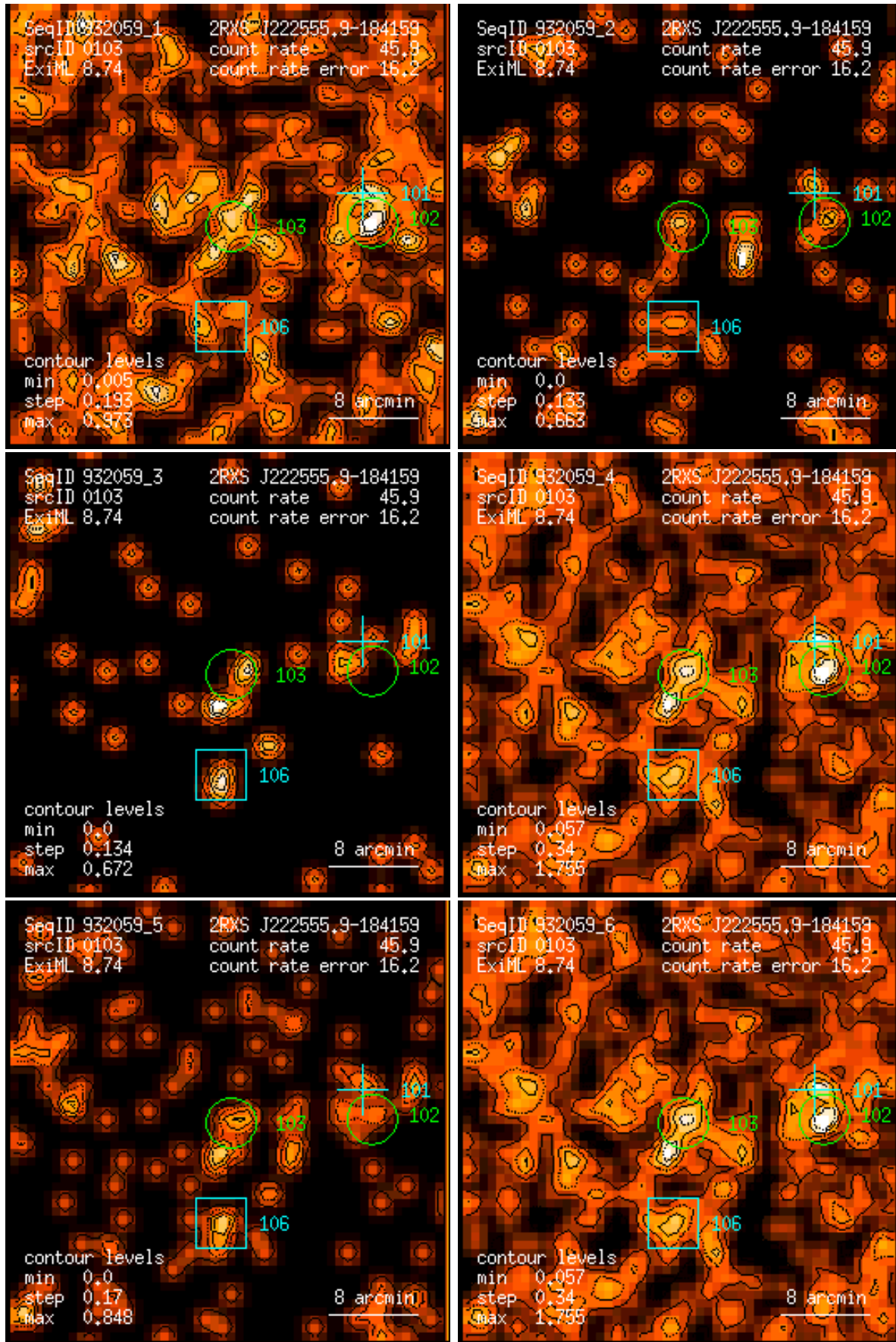
Figure 103: RASS 932059: detection 0103: band rate images, Gaussian filter: (1) PSPC channels 11 – 41, (2) 52 – 90, (3) 91 – 201, (4) 11 – 235, (5) 52 – 201, (6) 11 – 201. Broad band rates in counts/ks. Band rate contour levels in counts/ks/arcmin 2 .
