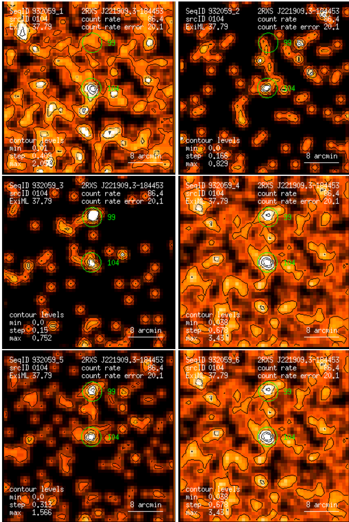
Figure 104: RASS 932059: detection 0104: band rate images, Gaussian filter: (1) PSPC channels 11 – 41, (2) 52 – 90, (3) 91 – 201, (4) 11 – 235, (5) 52 – 201, (6) 11 – 201. Broad band rates in counts/ks. Band rate contour levels in counts/ks/arcmin 2 .
