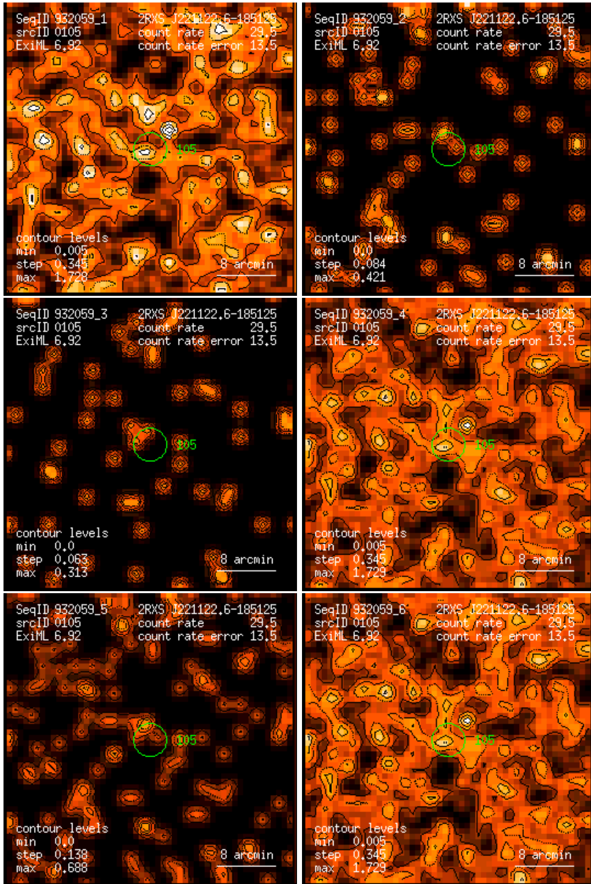
Figure 105: RASS 932059: detection 0105: band rate images, Gaussian filter: (1) PSPC channels 11 – 41, (2) 52 – 90, (3) 91 – 201, (4) 11 – 235, (5) 52 – 201, (6) 11 – 201. Broad band rates in counts/ks. Band rate contour levels in counts/ks/arcmin 2 .
