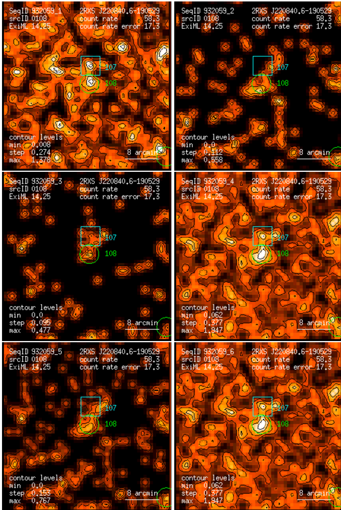
Figure 108: RASS 932059: detection 0108: band rate images, Gaussian filter: (1) PSPC channels 11 – 41, (2) 52 – 90, (3) 91 – 201, (4) 11 – 235, (5) 52 – 201, (6) 11 – 201. Broad band rates in counts/ks. Band rate contour levels in counts/ks/arcmin 2 .
