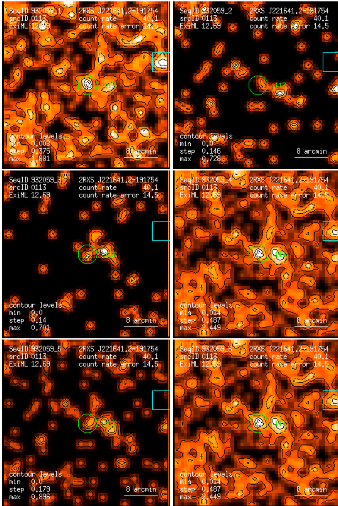
Figure 113: RASS 932059: detection 0113: band rate images, Gaussian filter: (1) PSPC channels 11 – 41, (2) 52 – 90, (3) 91 – 201, (4) 11 – 235, (5) 52 – 201, (6) 11 – 201. Broad band rates in counts/ks. Band rate contour levels in counts/ks/arcmin 2 .
