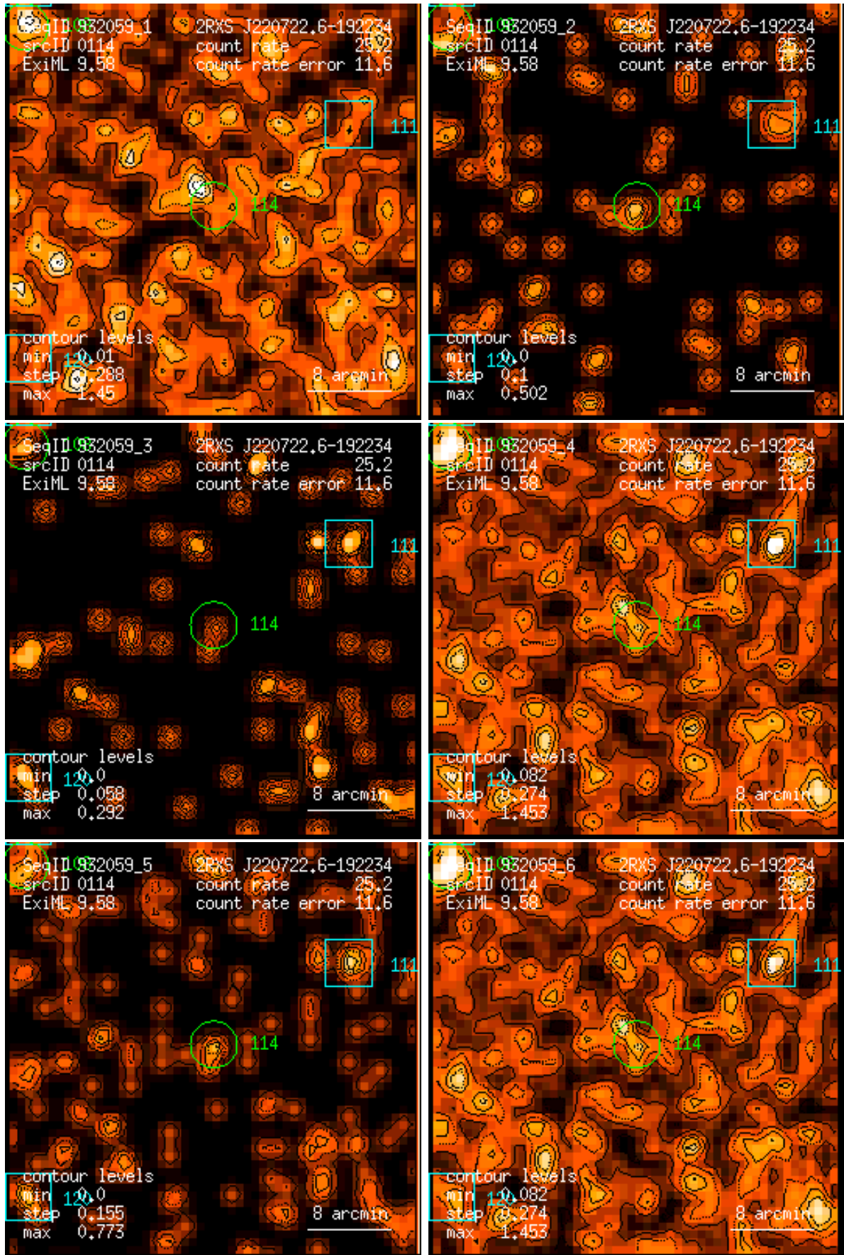
Figure 114: RASS 932059: detection 0114: band rate images, Gaussian filter: (1) PSPC channels 11 – 41, (2) 52 – 90, (3) 91 – 201, (4) 11 – 235, (5) 52 – 201, (6) 11 – 201. Broad band rates in counts/ks. Band rate contour levels in counts/ks/arcmin 2 .
