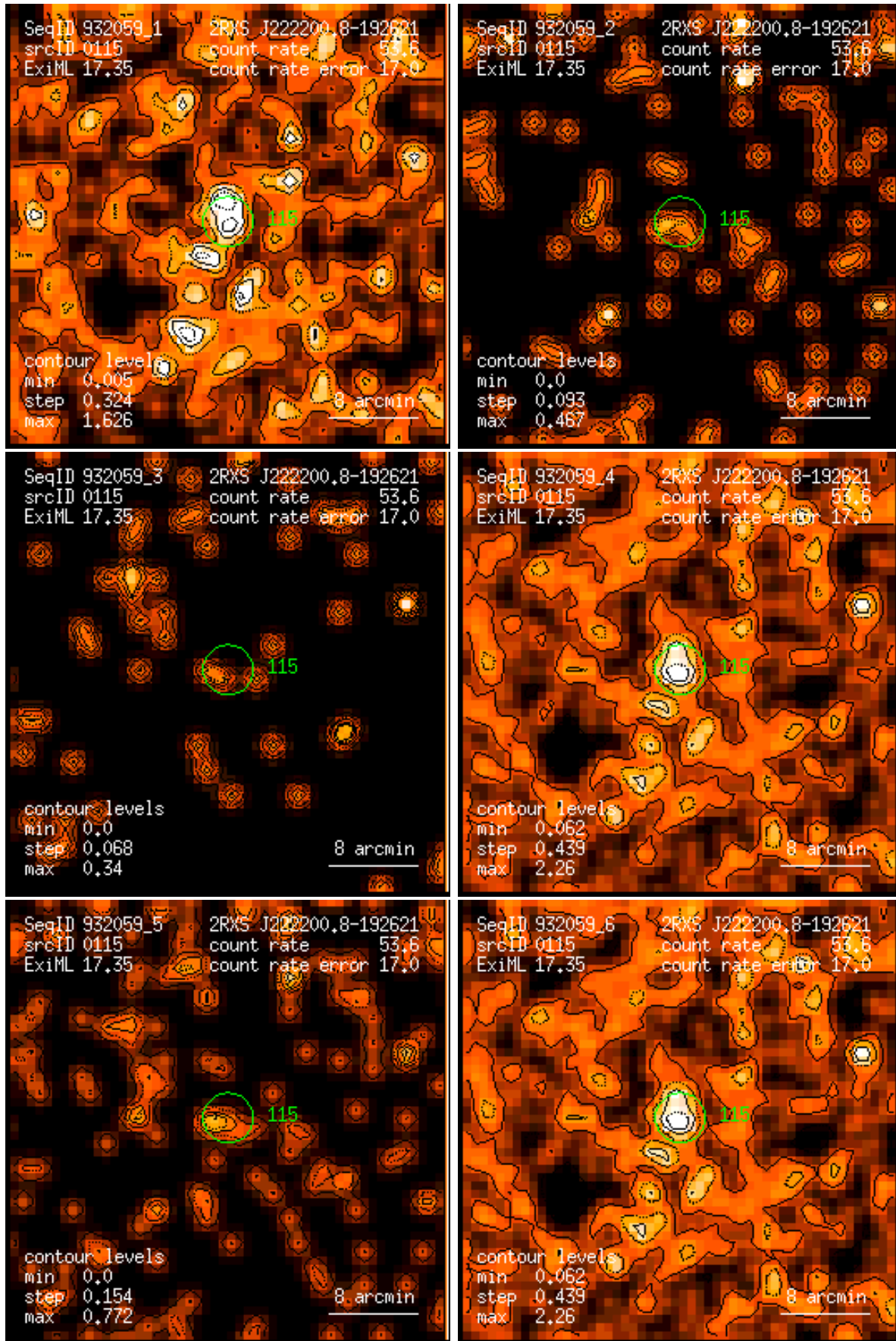
Figure 115: RASS 932059: detection 0115: band rate images, Gaussian filter: (1) PSPC channels 11 – 41, (2) 52 – 90, (3) 91 – 201, (4) 11 – 235, (5) 52 – 201, (6) 11 – 201. Broad band rates in counts/ks. Band rate contour levels in counts/ks/arcmin 2 .
