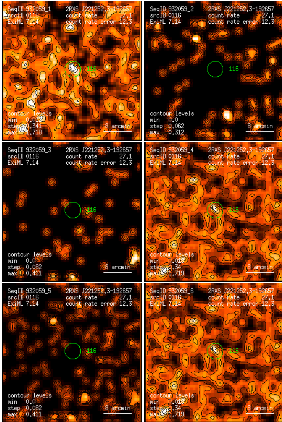
Figure 116: RASS 932059: detection 0116: band rate images, Gaussian filter: (1) PSPC channels 11 – 41, (2) 52 – 90, (3) 91 – 201, (4) 11 – 235, (5) 52 – 201, (6) 11 – 201. Broad band rates in counts/ks. Band rate contour levels in counts/ks/arcmin 2 .
