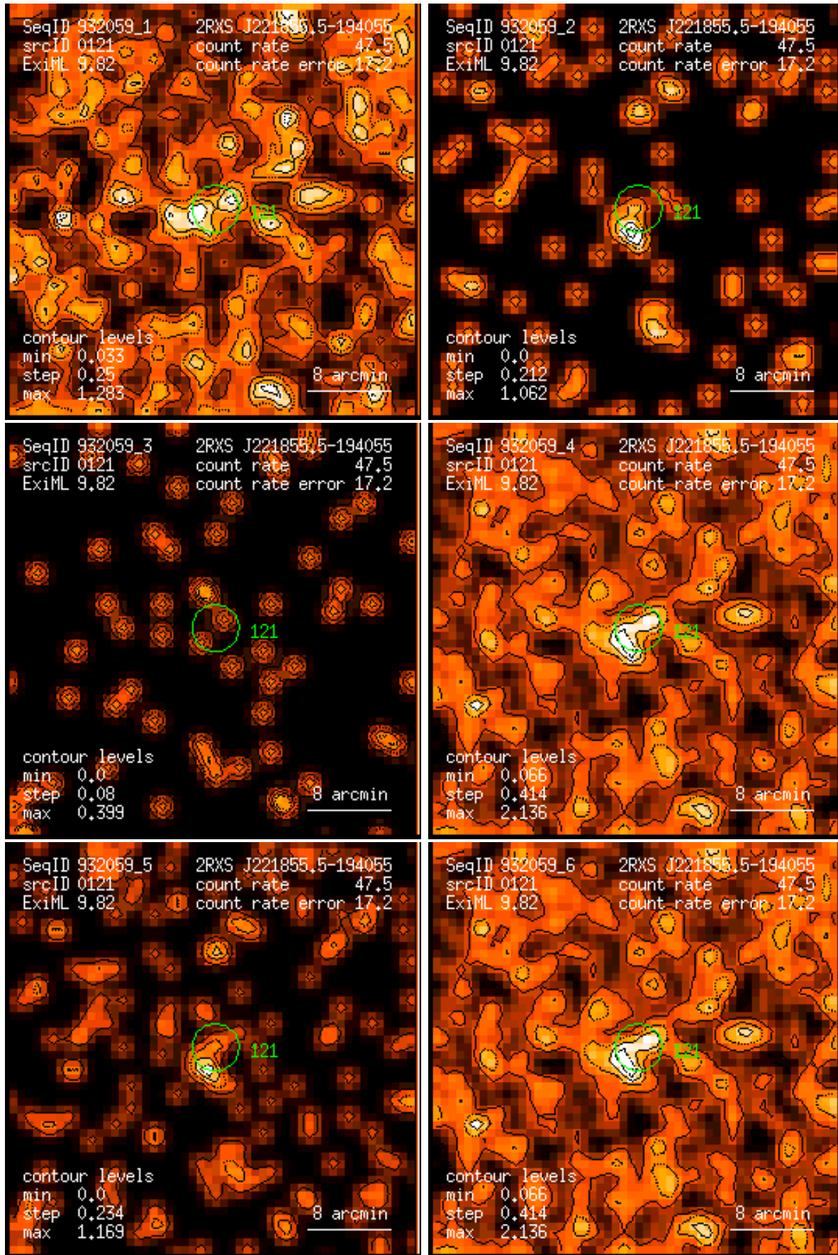
Figure 121: RASS 932059: detection 0121: band rate images, Gaussian filter: (1) PSPC channels 11 – 41, (2) 52 – 90, (3) 91 – 201, (4) 11 – 235, (5) 52 – 201, (6) 11 – 201. Broad band rates in counts/ks. Band rate contour levels in counts/ks/arcmin 2 .
