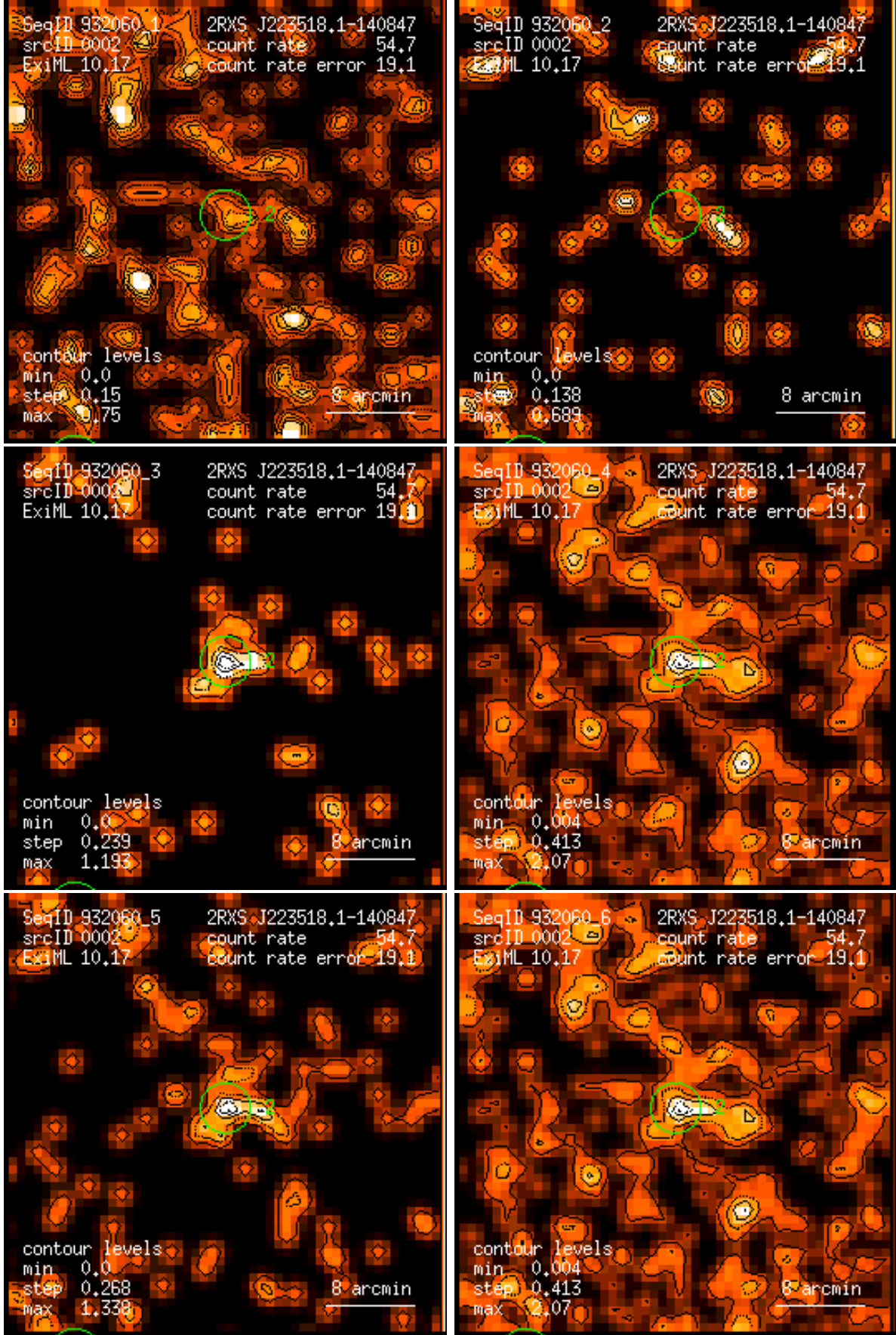
Figure 2: RASS 932060: detection 0002: band rate images, Gaussian filter: (1) PSPC channels 11 – 41, (2) 52 – 90, (3) 91 – 201, (4) 11 – 235, (5) 52 – 201, (6) 11 – 201. Broad band rates in counts/ks. Band rate contour levels in counts/ks/arcmin 2 .
